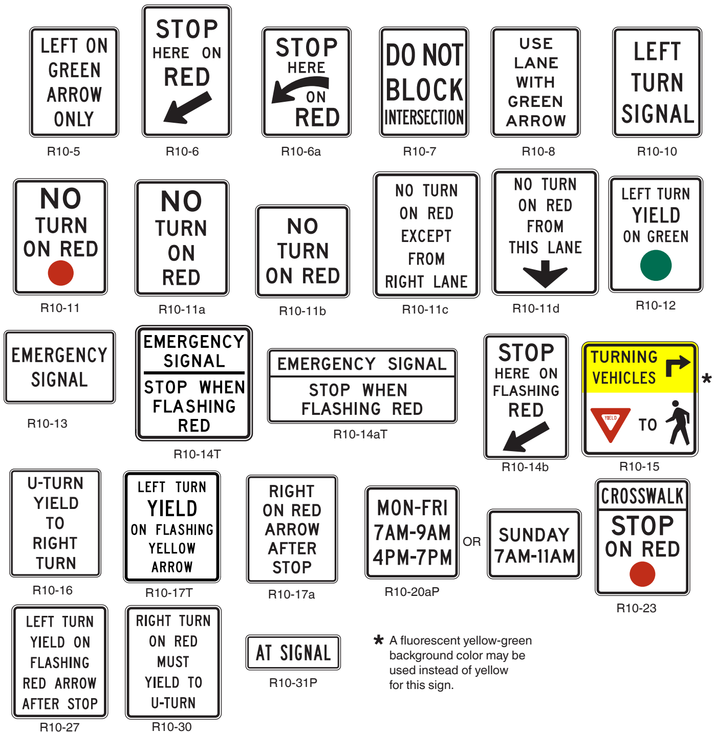
Figure 2B-27. Traffic Signal Signs and Plaques
