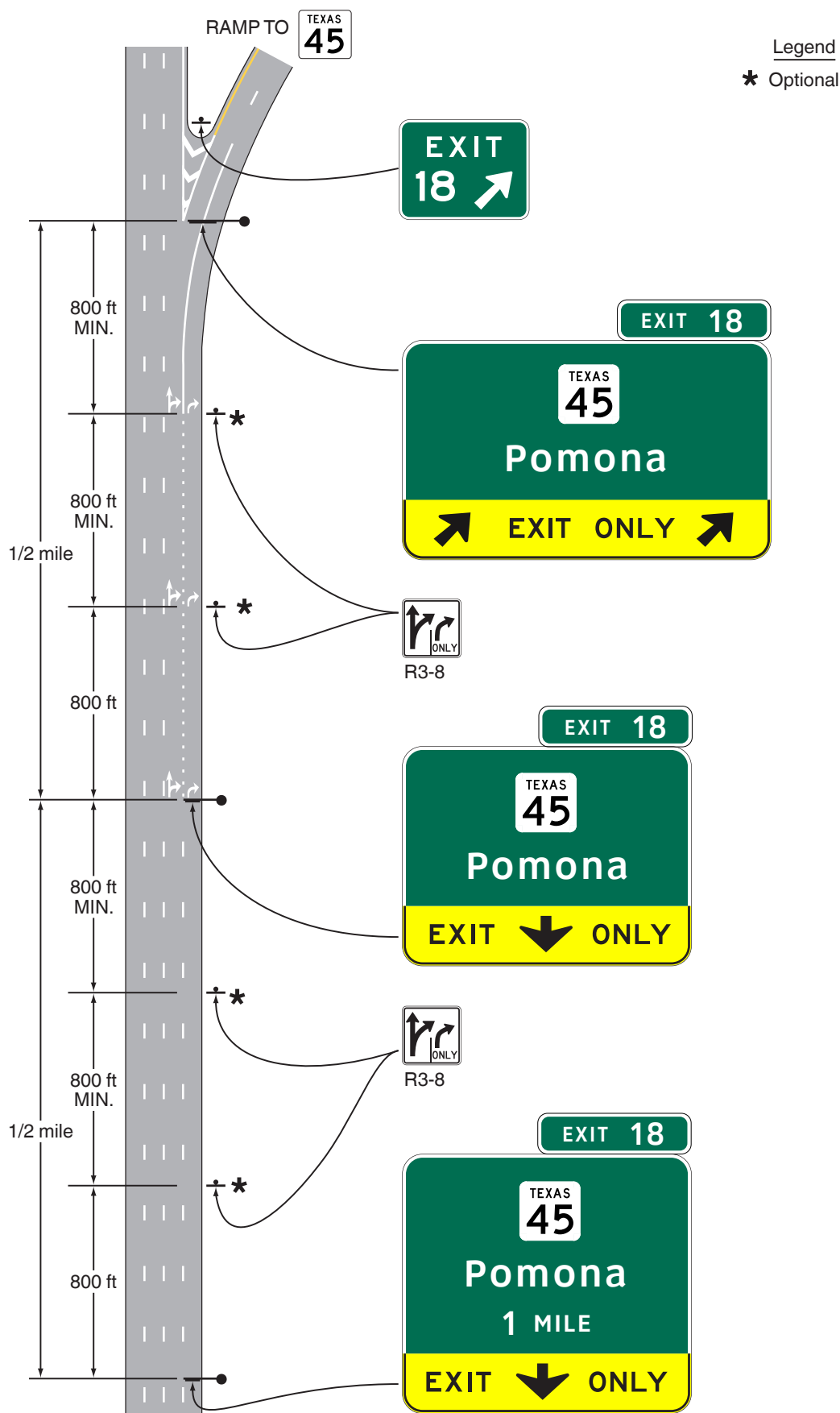
Figure 2E-11. Example of Signing for a Two-Lane Intermediate or Minor Interchange Exit with an Option Lane and a Dropped Lane
