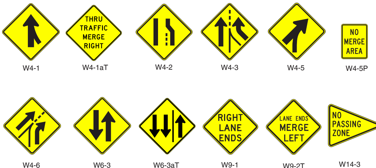
Figure 2C-8. Merging and Passing Signs and Plaques
