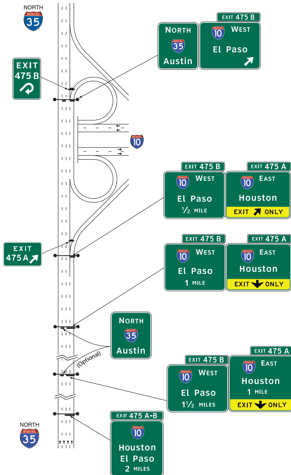
Figure 2E-36TB. Examples of Guide Signs for a Full Cloverleaf Interchange without Collector-Distributor Roadways
