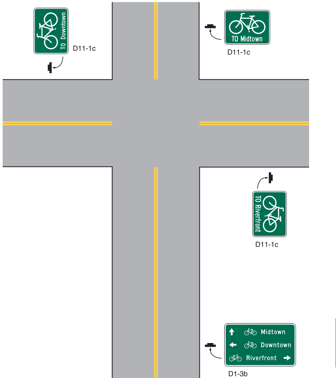
Figure 9B-6. Example of Bicycle Guide Signing
