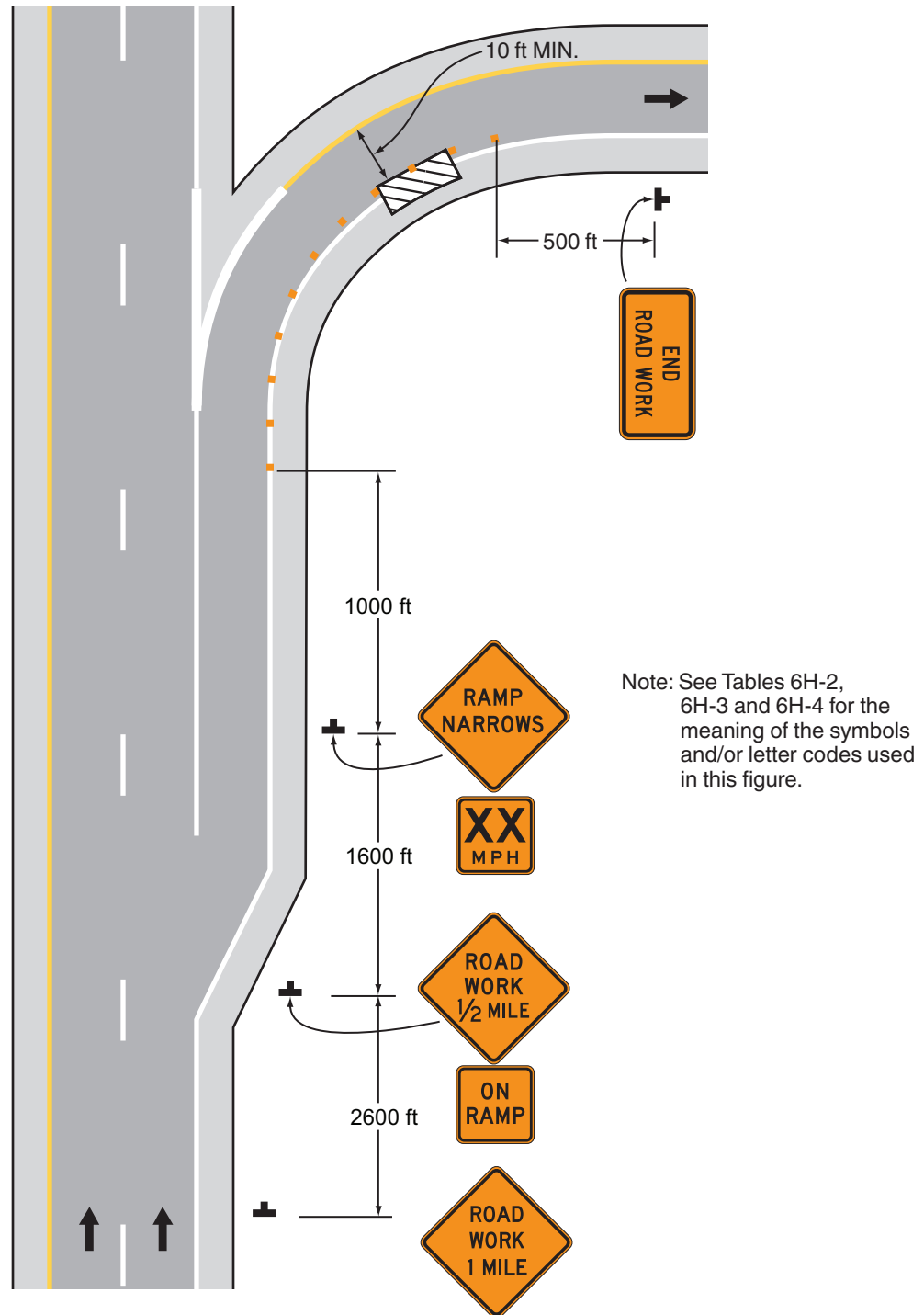
Typical Application 43
