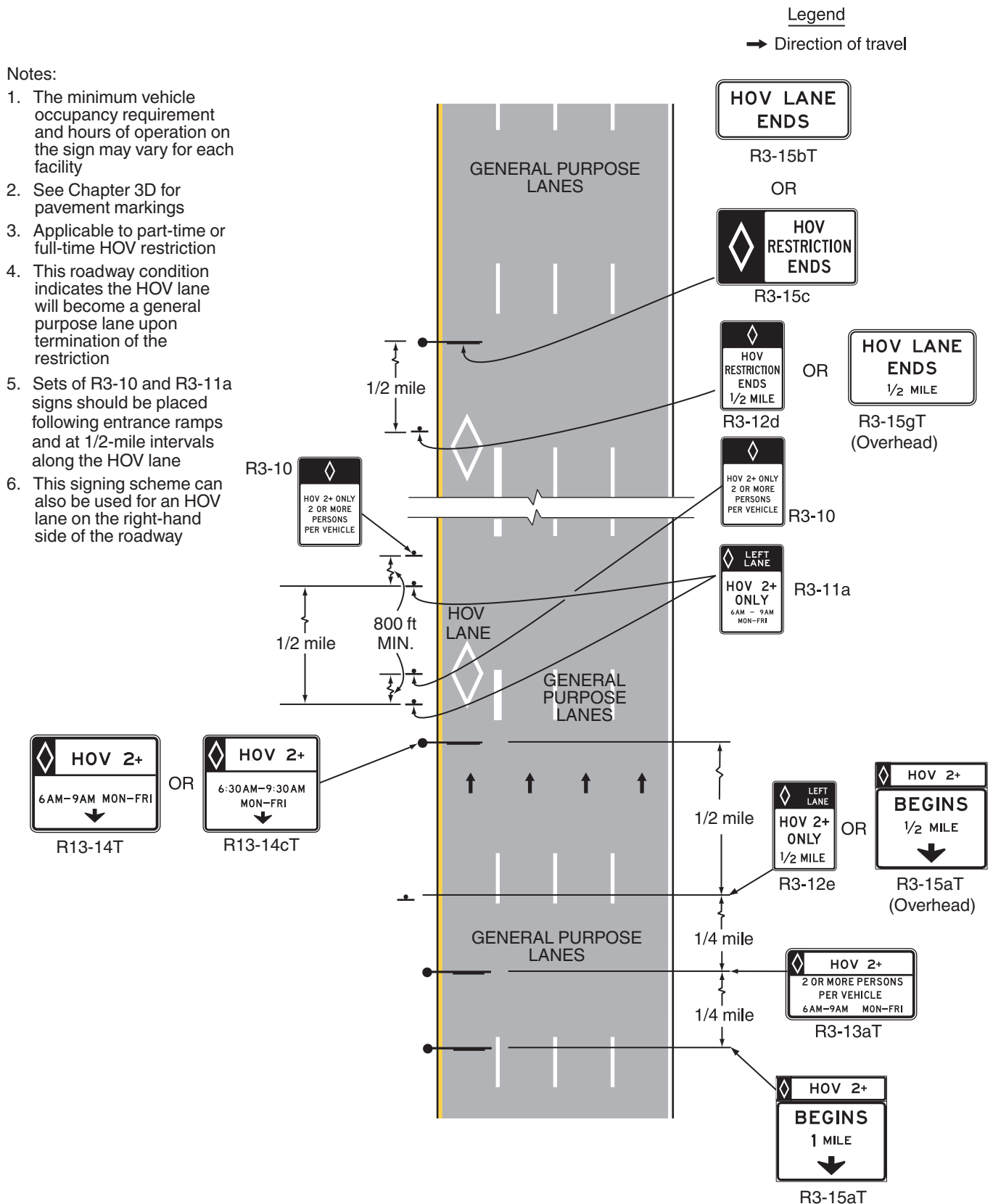
Figure 2G-3. Example of Signing for a General-Purpose Lane that Becomes a Continuous-Access Contiguous or Buffer-Separated HOV Lane
