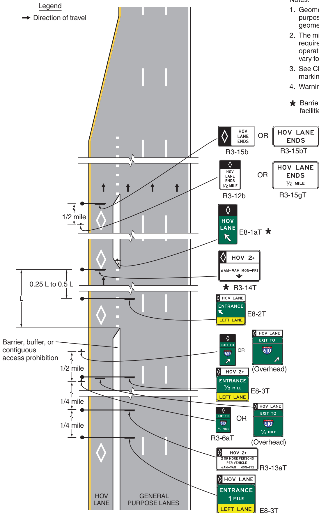
Figure 2G-10. Example of Signing for the Intermediate Entry to, Egress from, and End of Access-Restricted HOV Lanes
