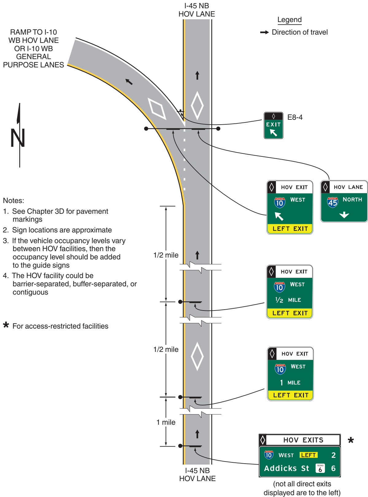
Figure 2G-16. Examples of Guide Signs for a Direct Access Ramp between HOV Lanes on Separate Freeways
