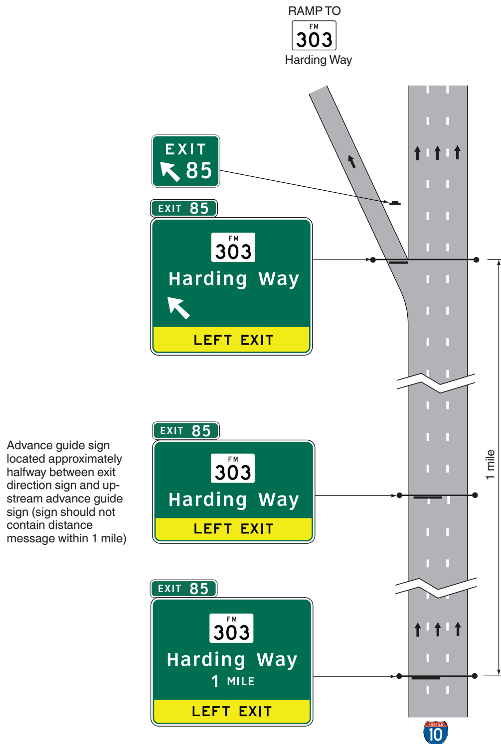
Figure 2E-16TA. Guide Signs for a Single-Left Lane Exit
