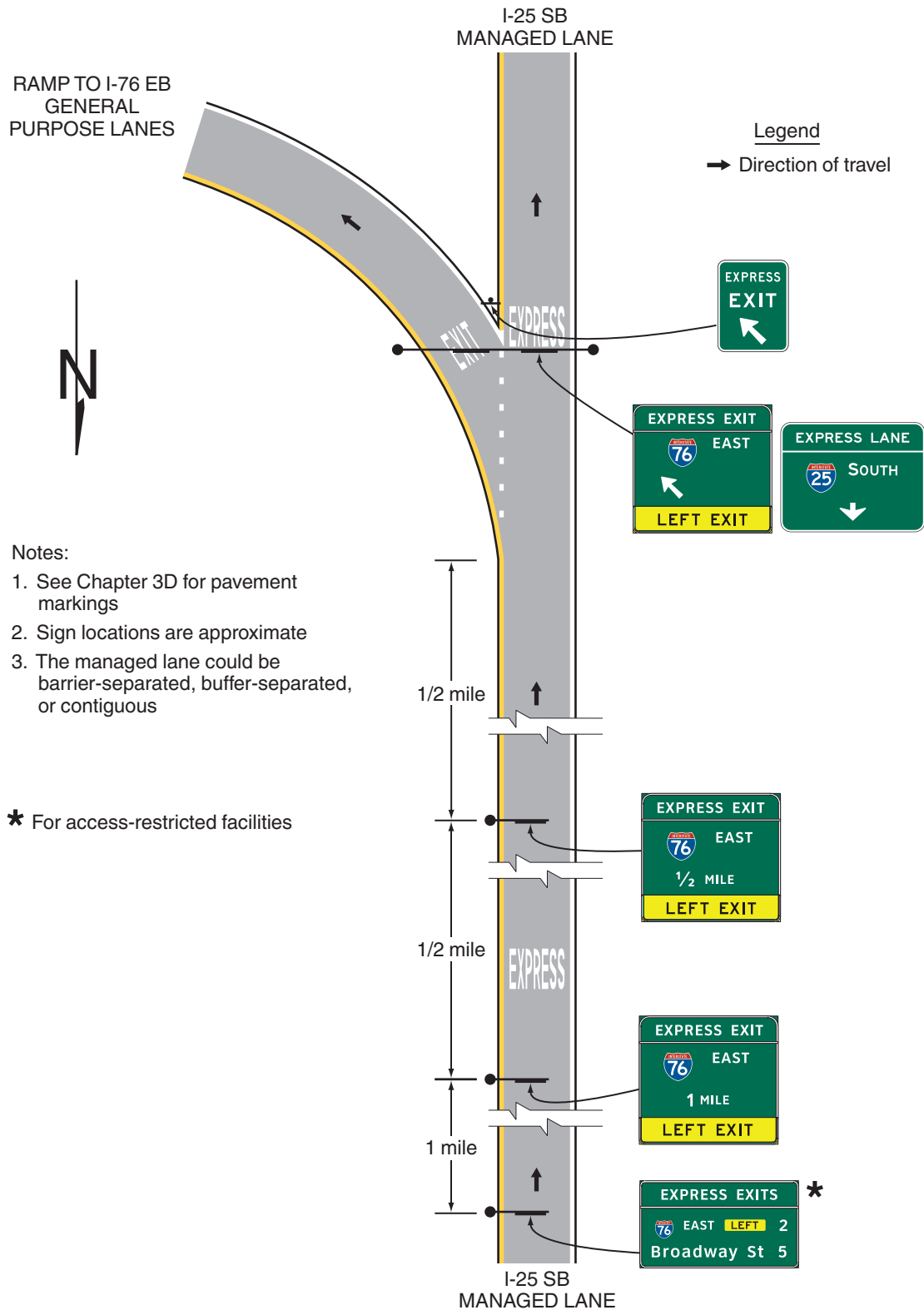
Figure 2G-27TA. Examples of Guide Signs for a Direct Access Ramp to General Purpose Lanes
