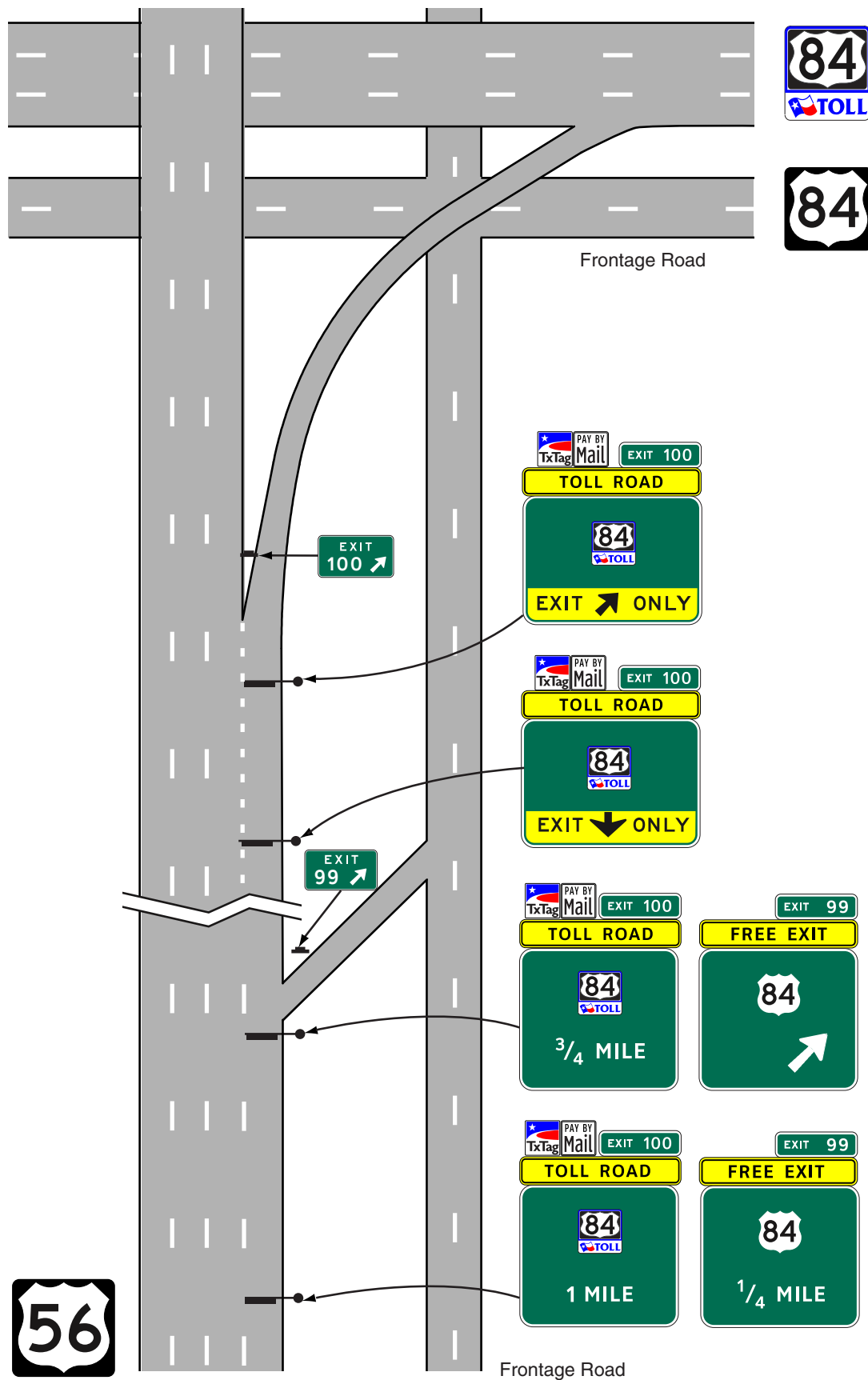
Figure 2F-6TA. Examples of Guide Signs from the Main Lane to a Toll Road
