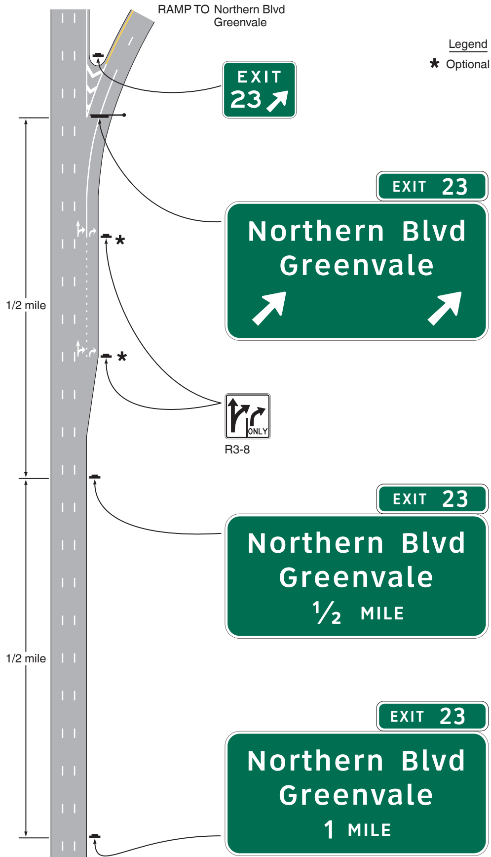
Exit with Option and Auxiliary Lanes
