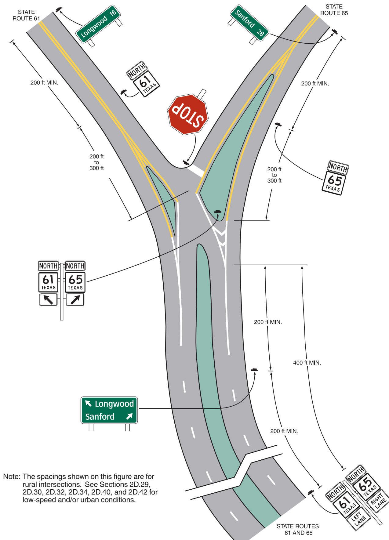
Figure 2D-6. Illustration of Directional Assemblies and Other Route Signs (for One Direction of Travel Only) (Sheet 4 of 4)
