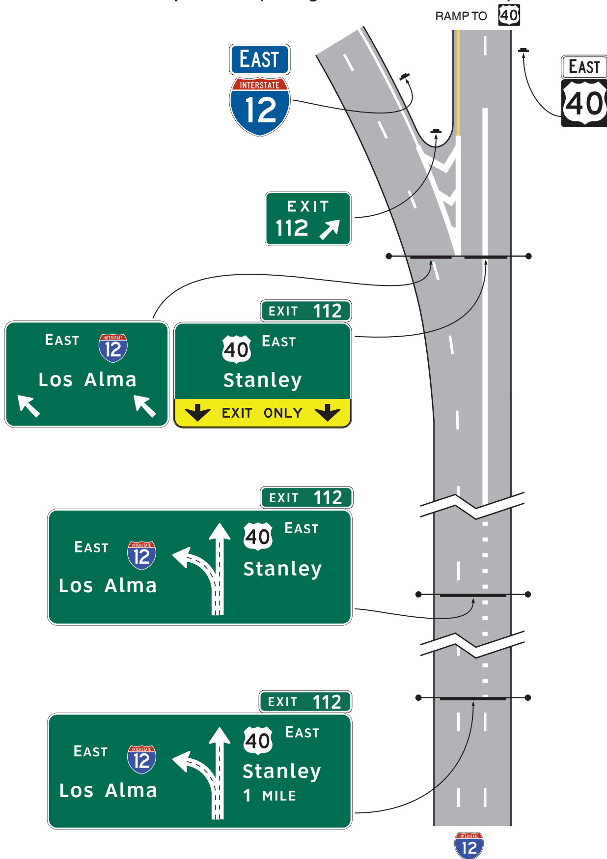
Figure 2E-9. Diagrammatic Guide Signs for a Two-Lane Exit to the Right with an Option Lane (Through Lanes Curve to the Left)
