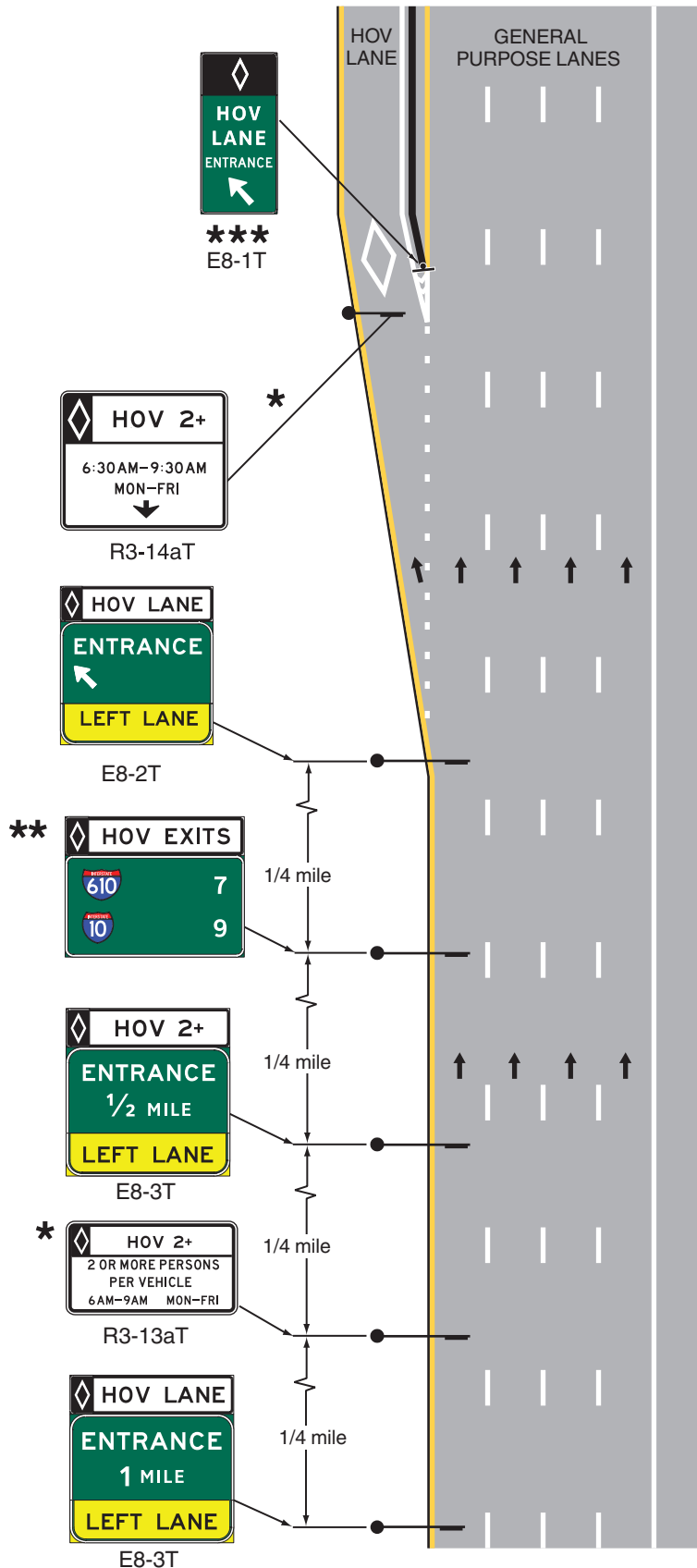
Figure 2G-8. Example of Signing for an Entrance to Access-Restricted HOV Lanes
