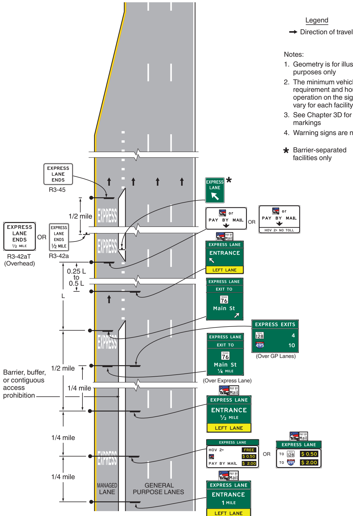
Figure 2G-24T. Example of Signing for the Intermediate Entry to, Egress from, and End of Access-Restricted Priced Express Lanes
