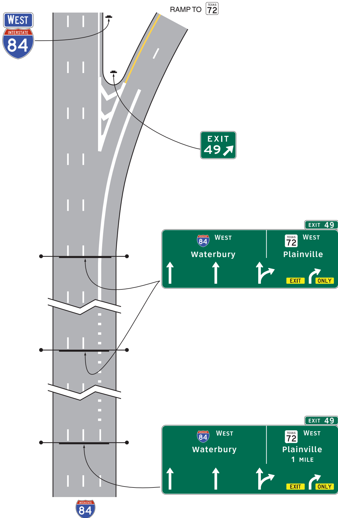
Figure 2E-4. Overhead Arrow-per-Lane Guide Signs for a Two-Lane Exit to the Right with an Option Lane
