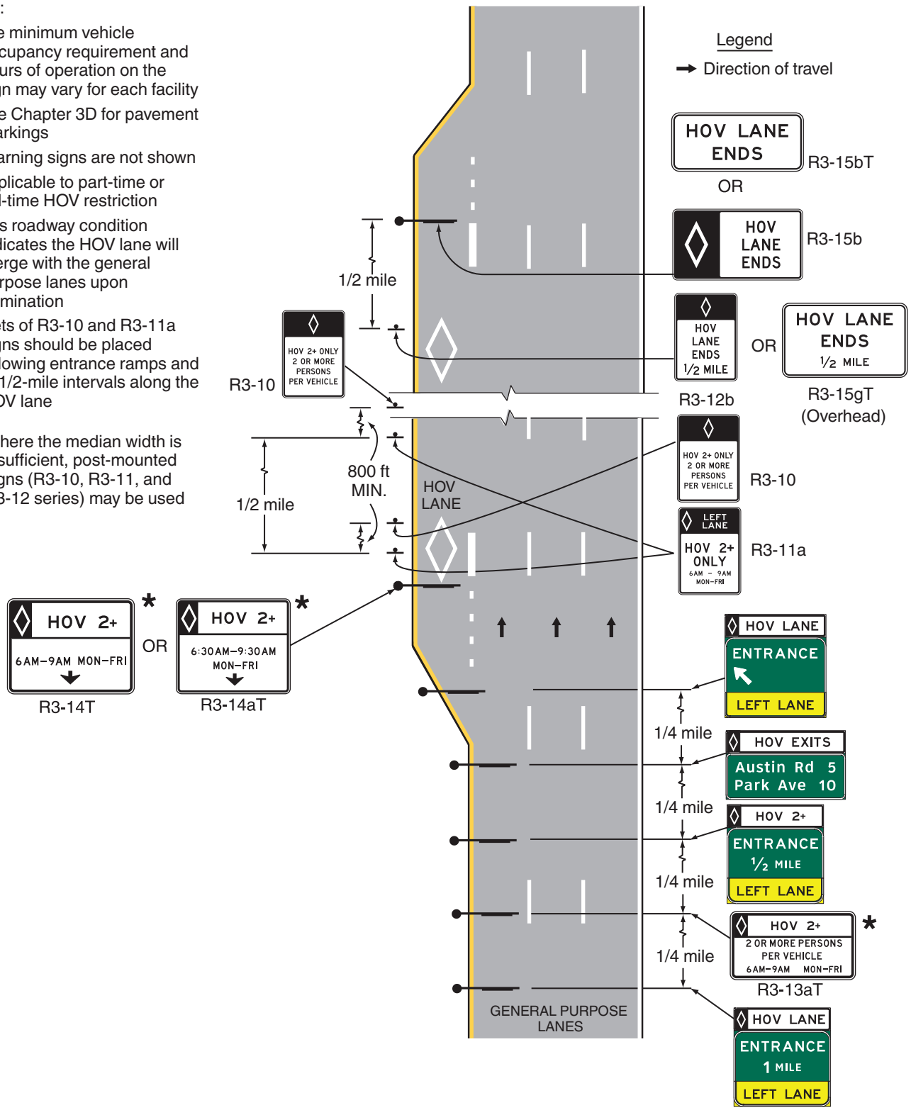
Figure 2G-2. Example of Signing for an Added Continuous-Access Contiguous or Buffer-Separated HOV Lane
