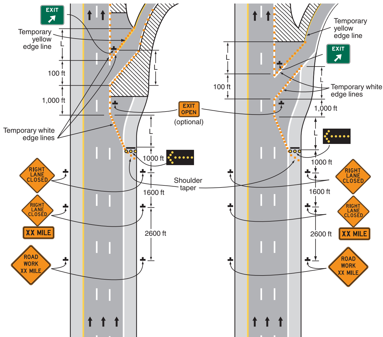
Typical Application 42
