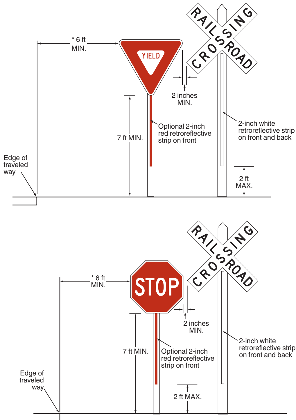
Figure 8B-3. Crossbuck Assembly with a YIELD or STOP Sign on a Separate Sign Support
