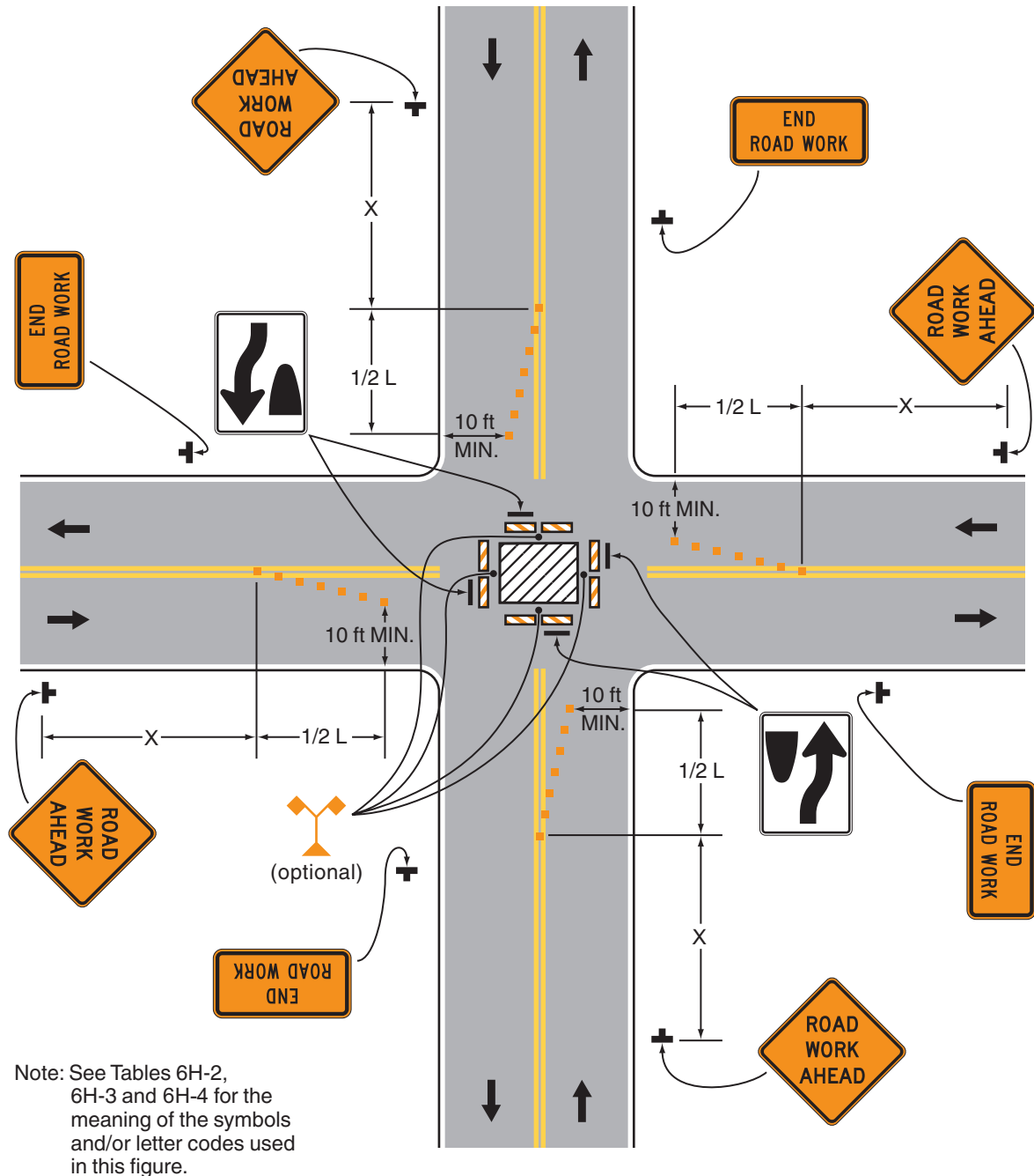
Typical Application 26
