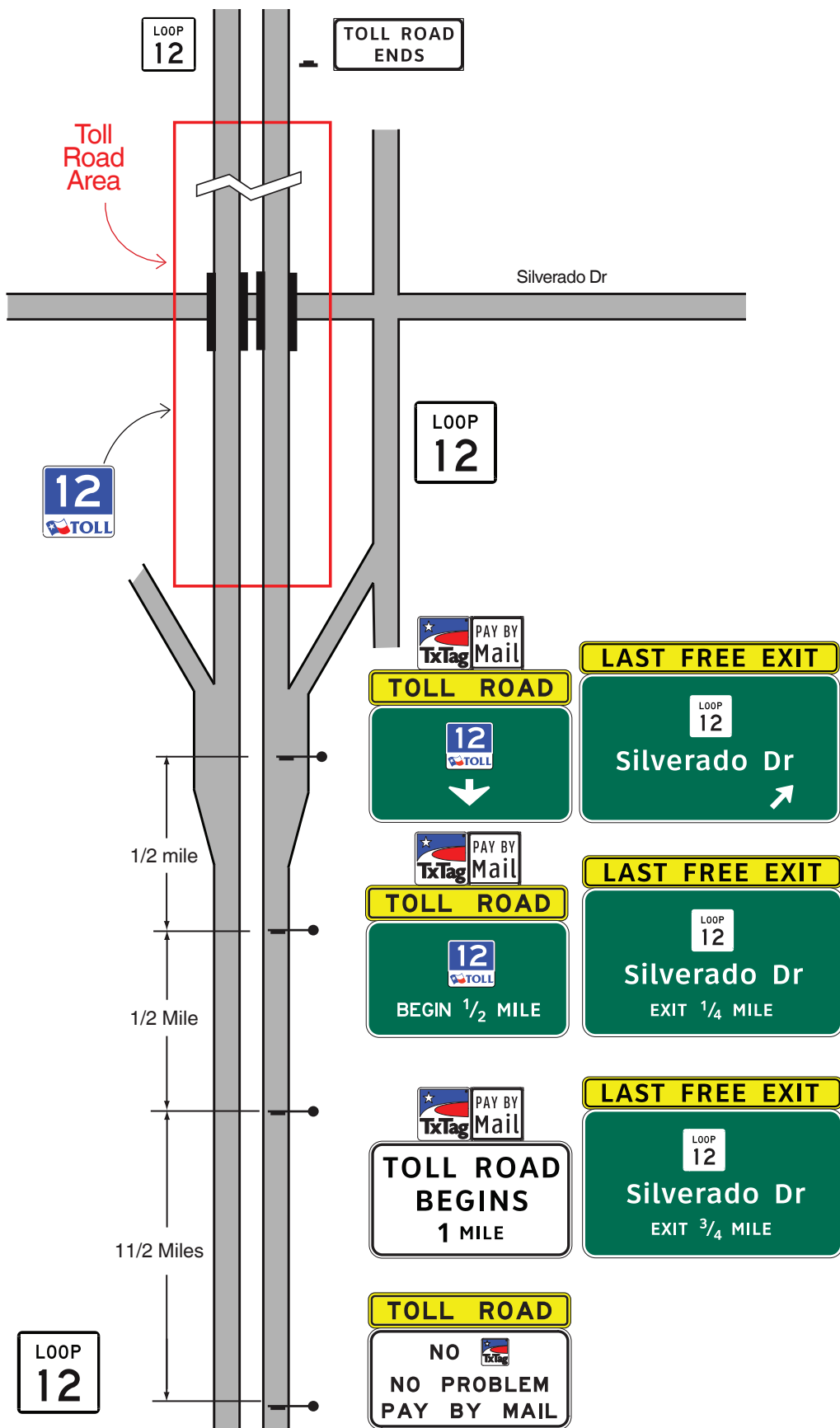
Figure 2F-7TA. Non-Toll Roadway Converts to Toll Roadway
