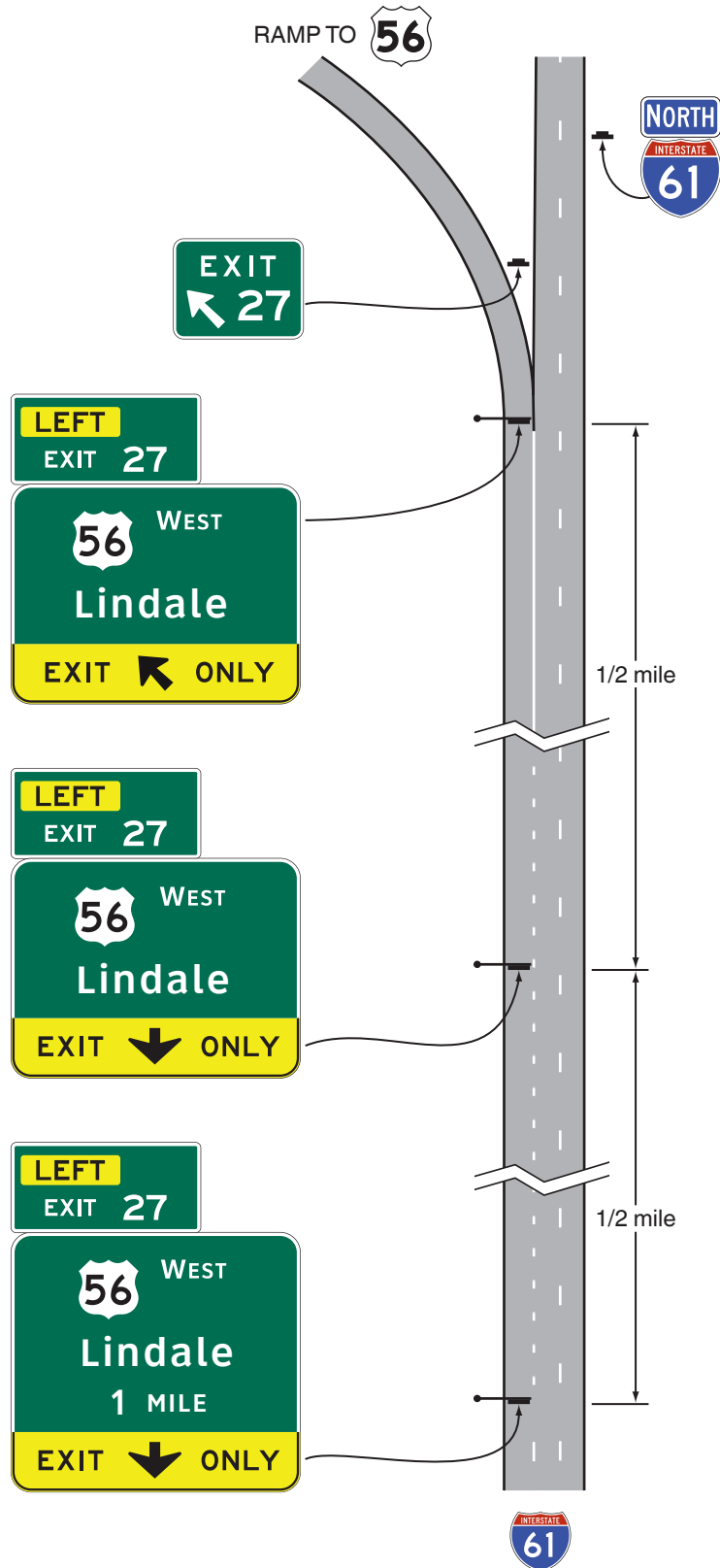
Figure 2E-15. Guide Signs for a Single-Lane Exit to the Left with a Dropped Lane
