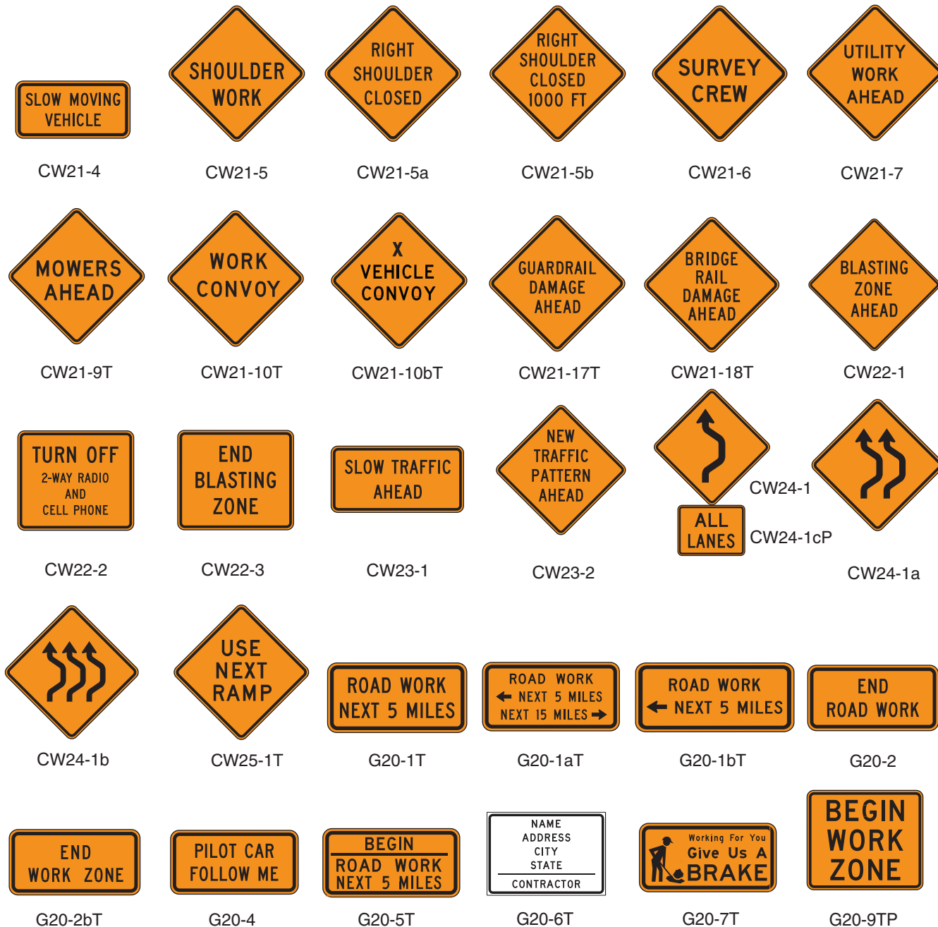
Figure 6F-4. Warning Signs and Plaques in Temporary Traffic Control Zones (Sheet 3 of 3)
