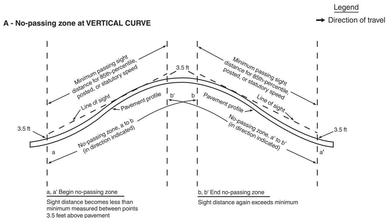
Figure 3B-4. Method of Locating and Determining the Limits of No-Passing Zones at Curves
