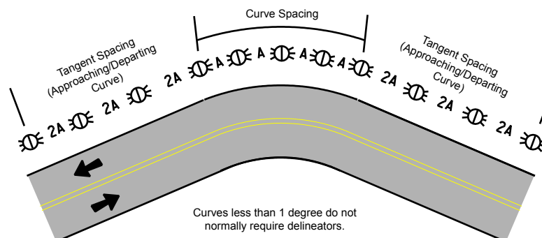
Figure 3F-T2. Suggested Spacing for Highway Delineators on Horizontal Curves
