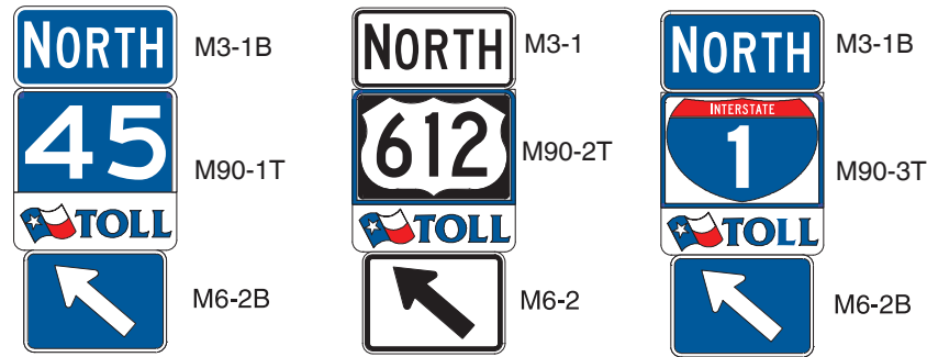
Figure 2F-3TA. Examples of TOLL Route Small Sign Assemblies
