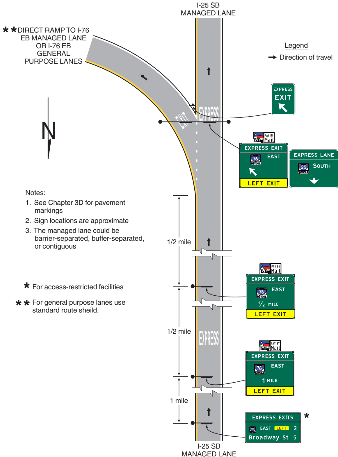
Figure 2G-27. Examples of Guide Signs for a Direct Access Ramp to Managed Lane
