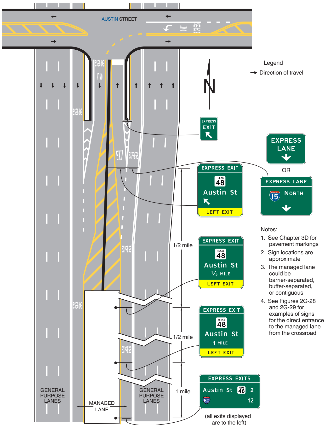
Figure 2G-26T. Examples of Guide Signs for Direct Managed Lane Entrance and Exit Ramps
