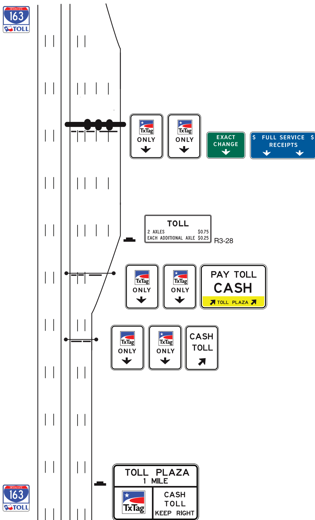
Figure 2F-10TA. Examples of Mainline Toll Plaza Approach and Canopy Signing
