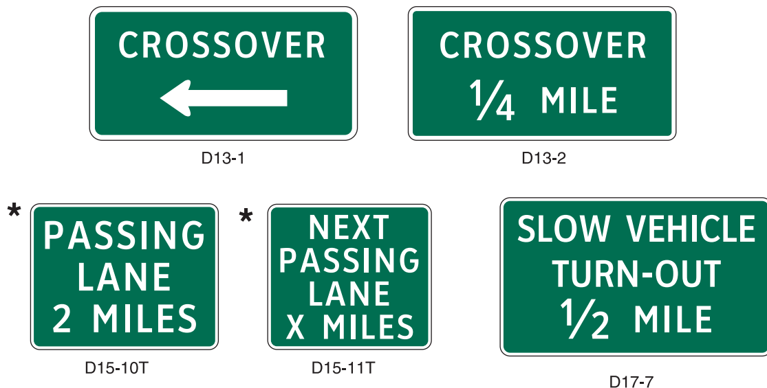
Figure 2D-21. Crossover, Passing Lane, and Slow Vehicle Signs
