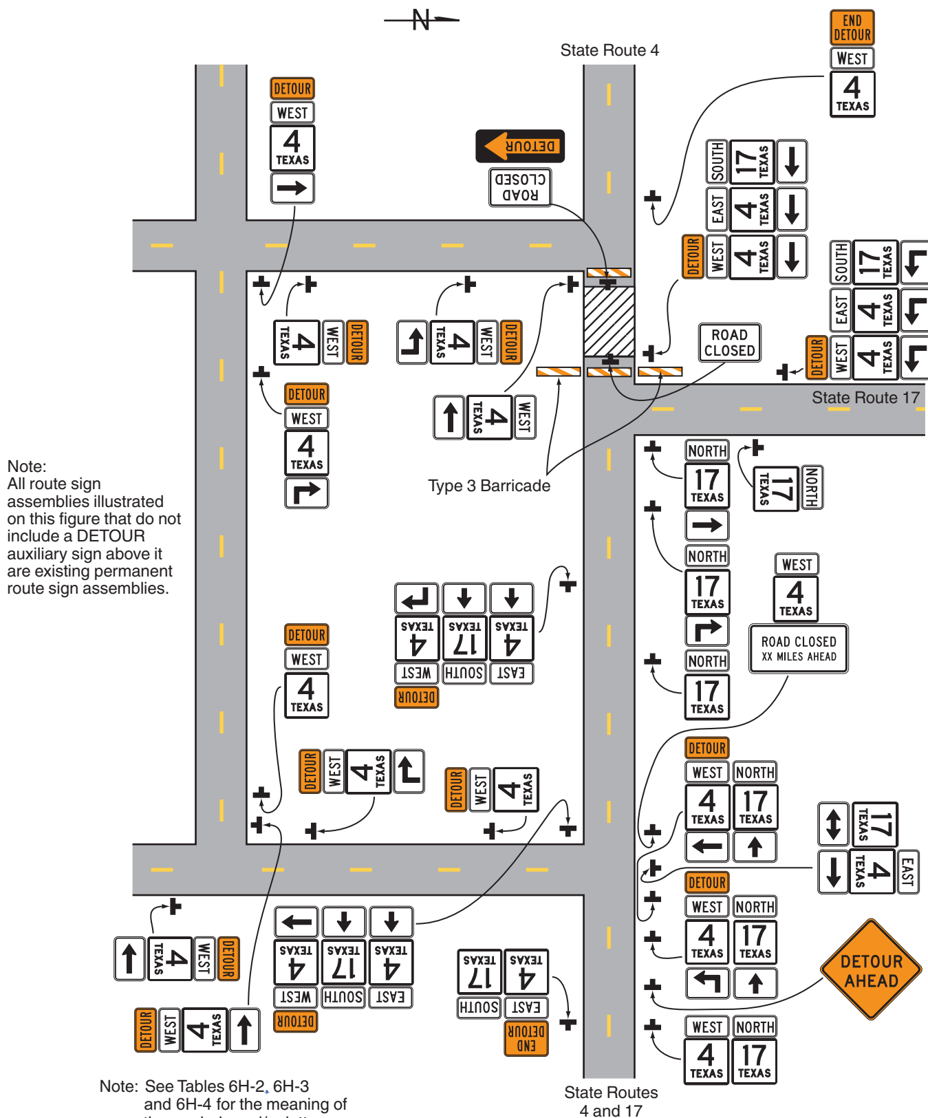
Typical Application 9
