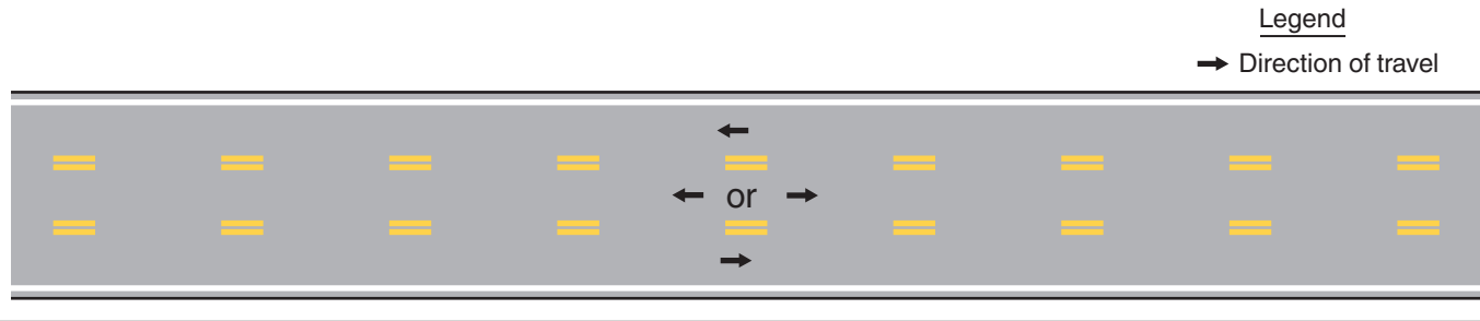
Figure 3B-6. Example of Reversible Lane Marking Application
