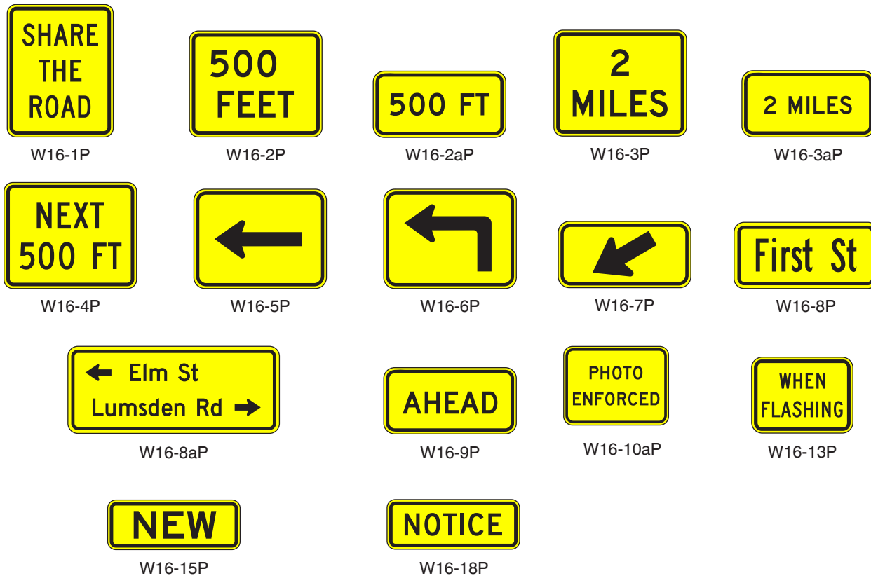
Figure 2C-12. Supplemental Warning Plaques
