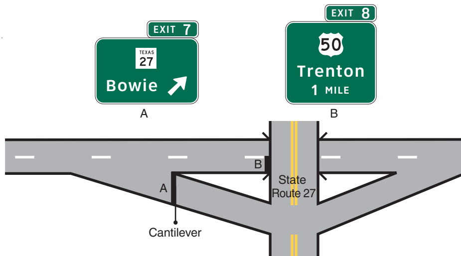
Figure 2E-1. Example of Guide Sign Spreading
