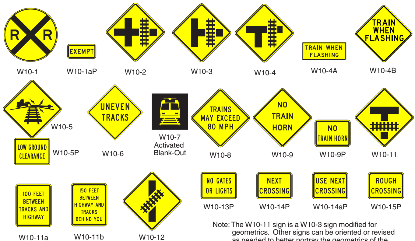
Figure 8B-4. Warning Signs and Plaques for Grade Crossings
