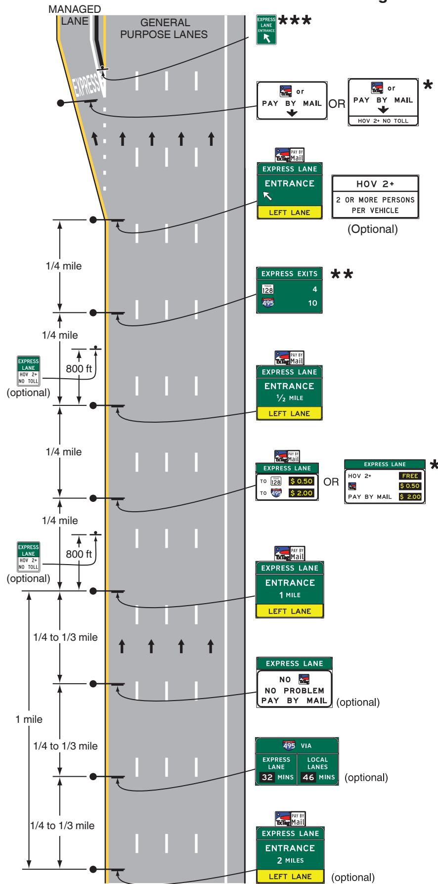
Figure 2G-21T. Example of Signing for the Entrance
