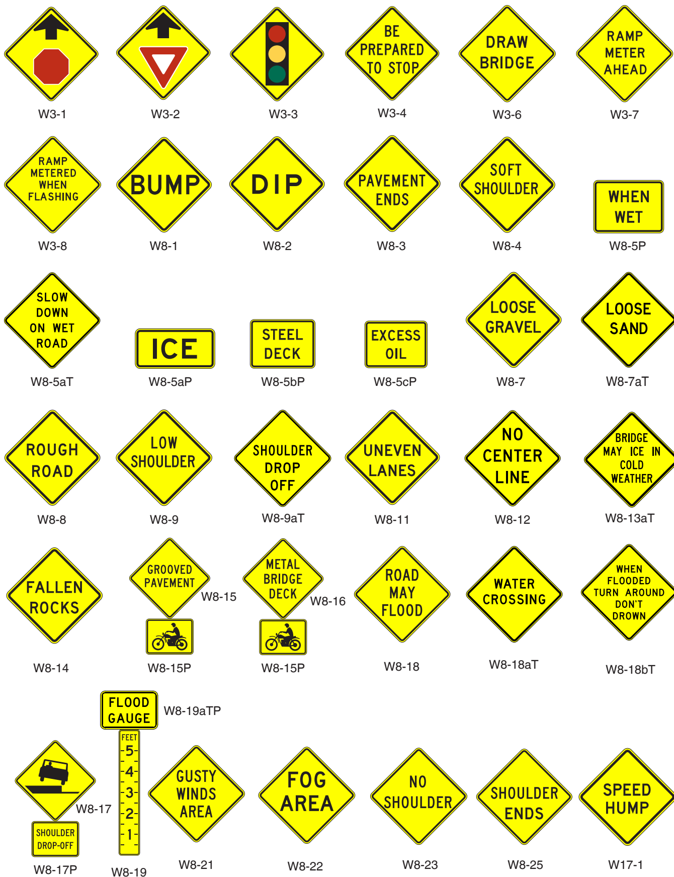
Figure 2C-6. Roadway and Weather Condition and Advance Traffic Control Signs and Plaques (1 of 2)
