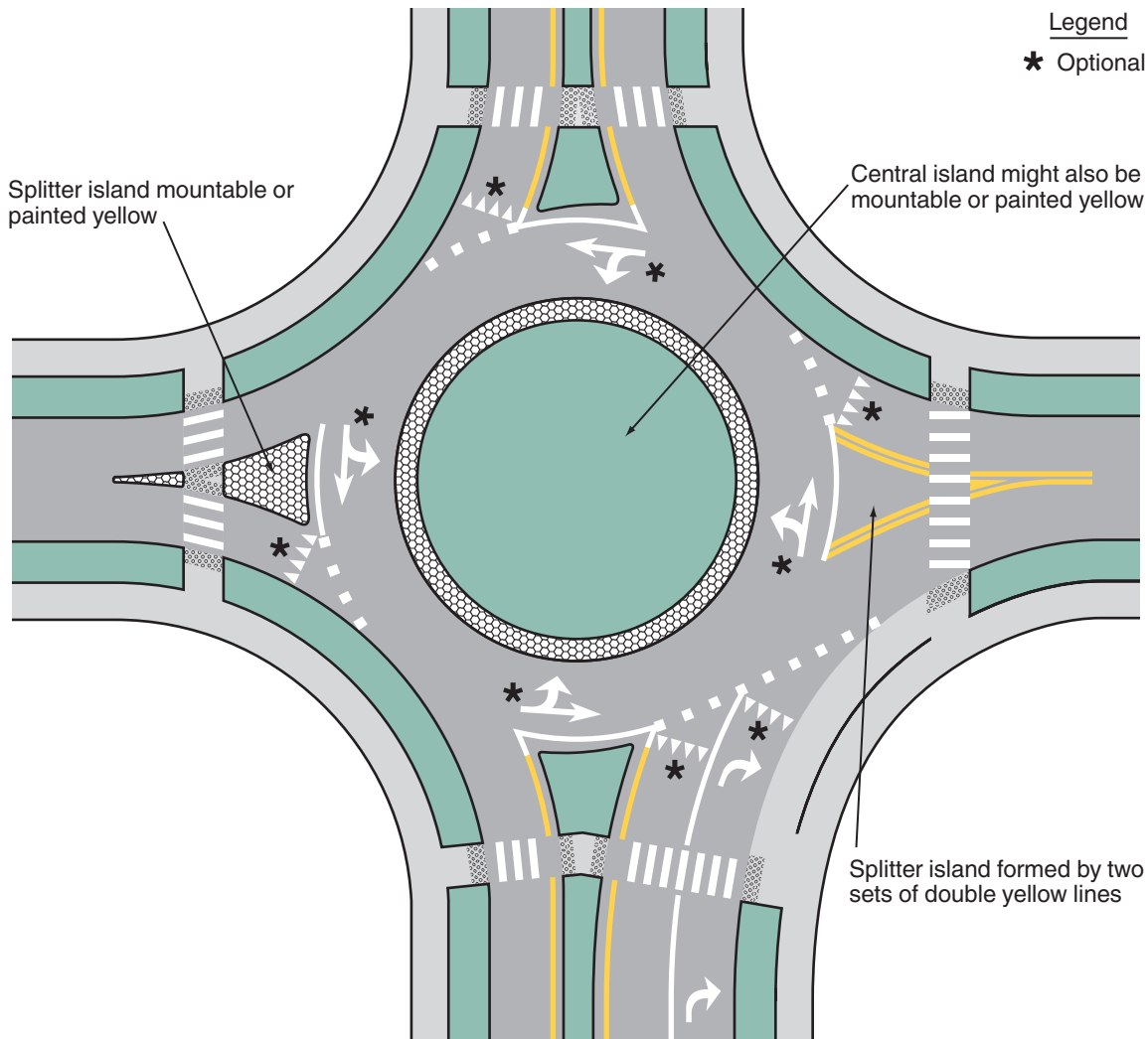
Figure 3C-3. Example of Markings for a One-Lane Roundabout
