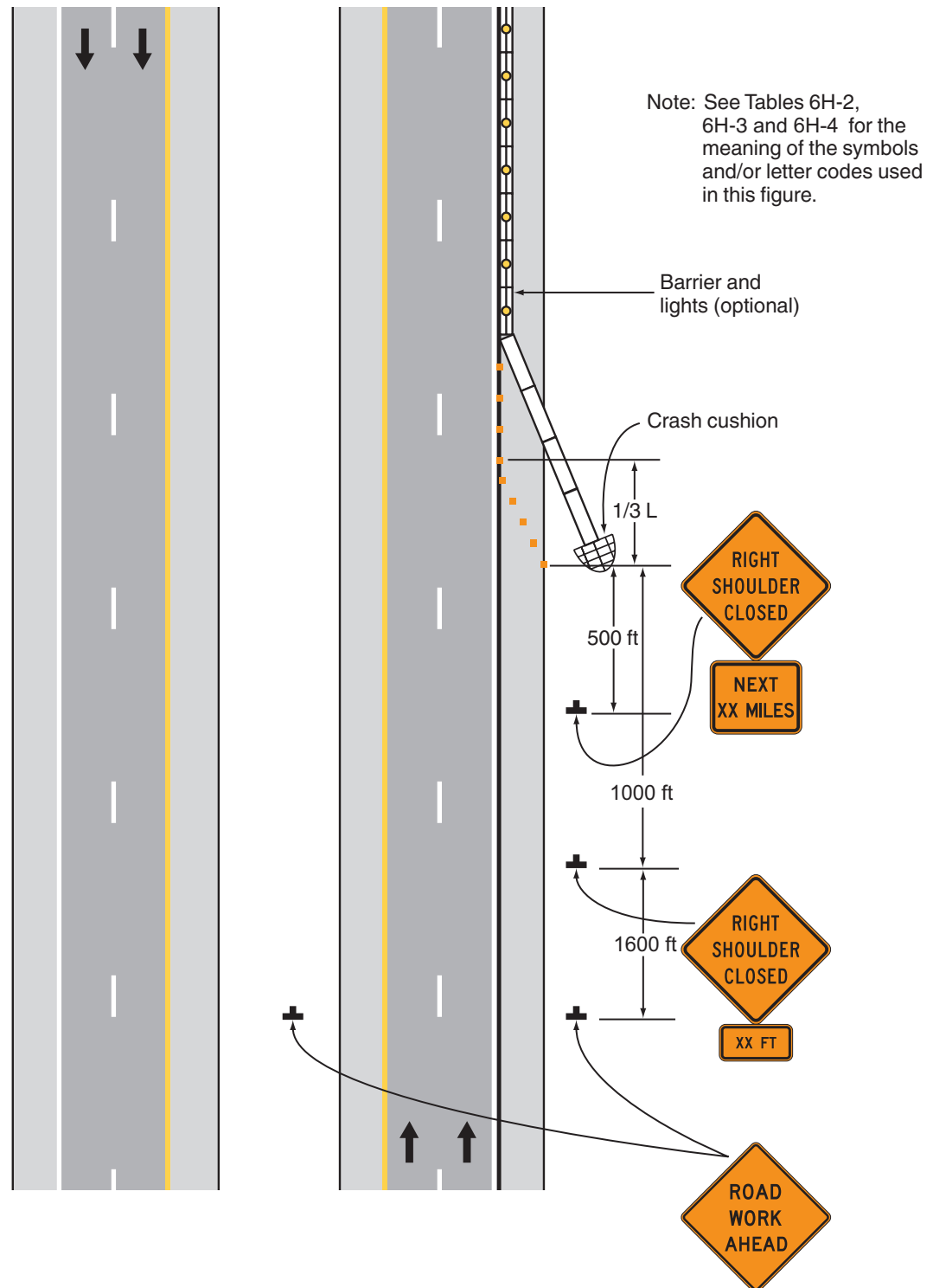
Typical Application 5
