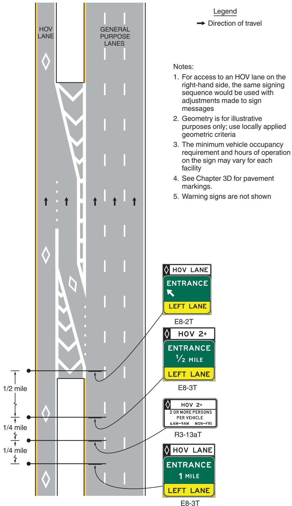
Figure 2G-9. Example of Signing for an Intermediate Entry to a Barrier- or Buffer-Separated HOV Lane
