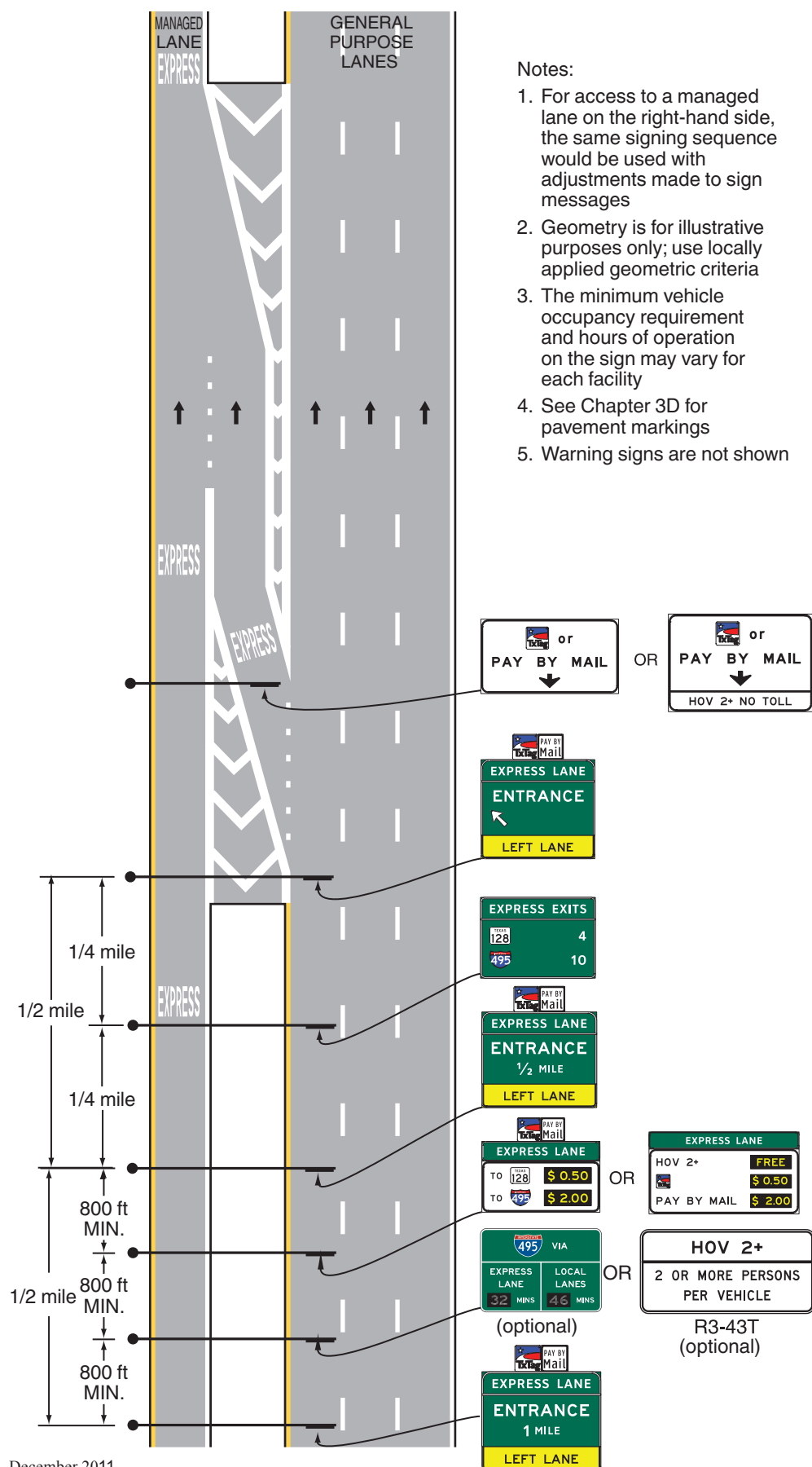
Figure 2G-23T. Example of Signing for an Intermediate Entry to a Barrier- or Buffer-Separated Priced Managed Lane
