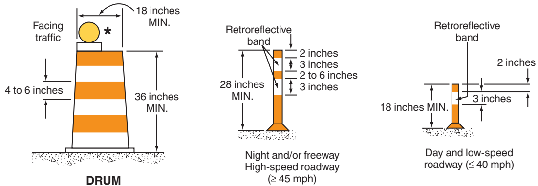
Figure 6F-7. Channelizing Devices (Sheet 1 of 2)
