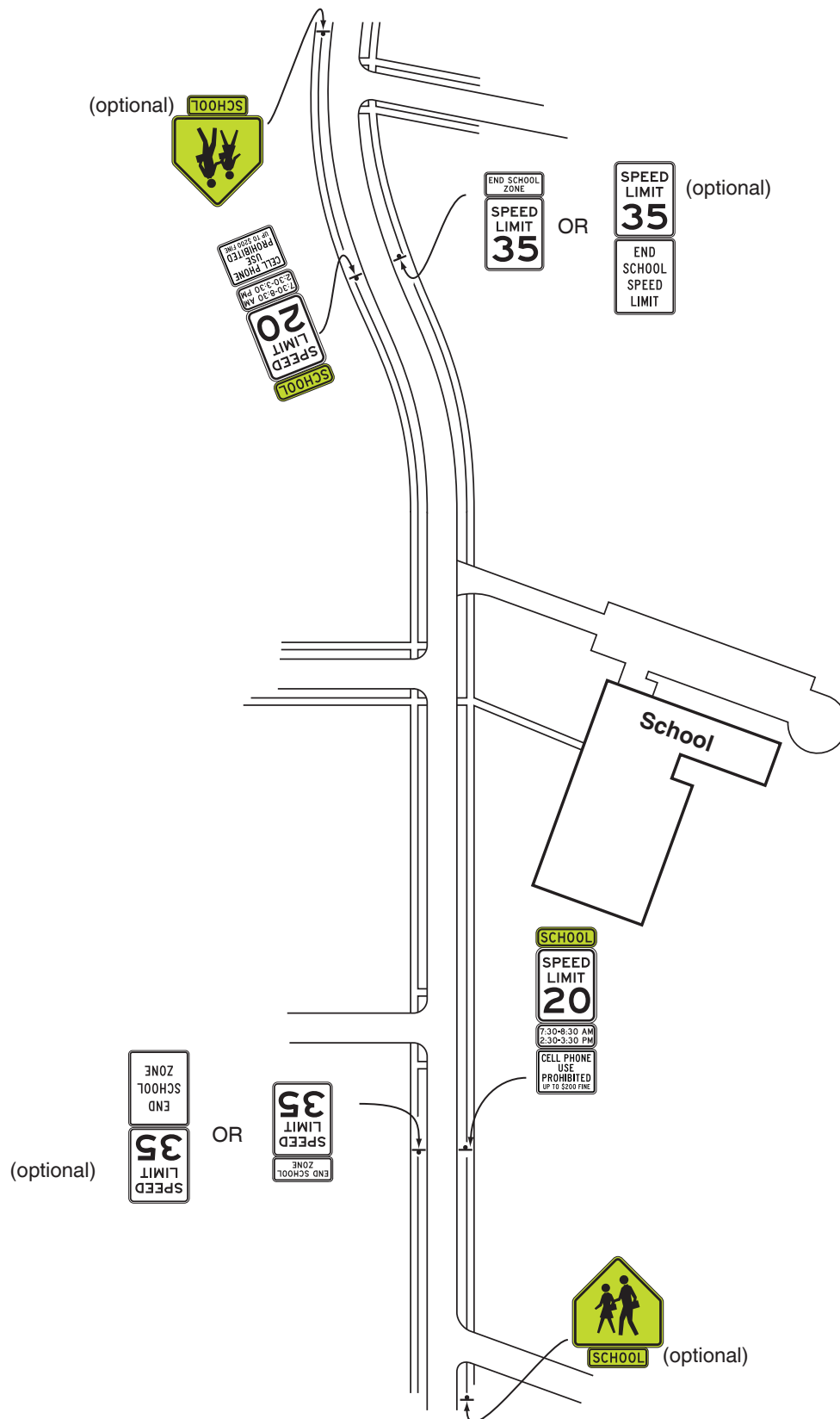
Figure 7B-3. Example of Signing for a Cell Phone Use Prohibited with a School Speed Limit
