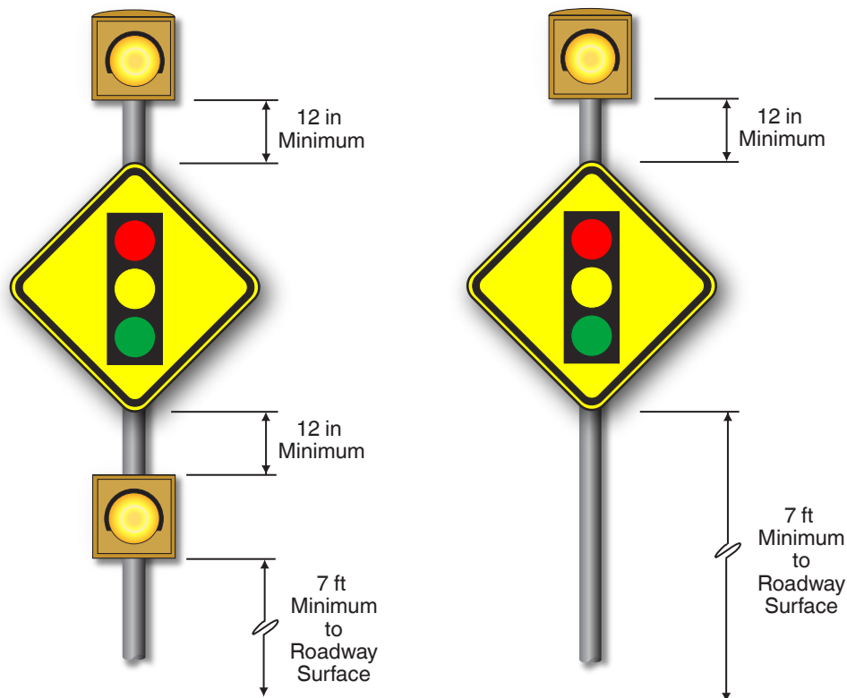
Figure 4L-1T Typical Warning Sign and Hazard Identification Beacon
