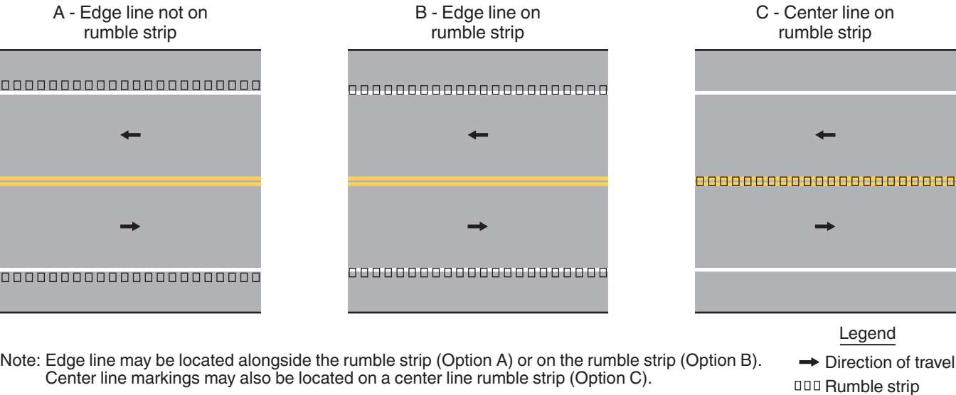
Figure 3J-1. Examples of Longitudinal Rumble Strip Markings
