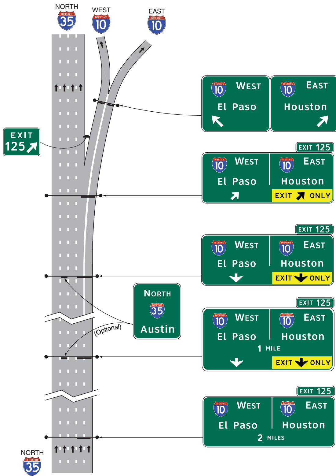
Figure 2E-2TC. Overhead Down Arrow for Option Right Lane Exit
