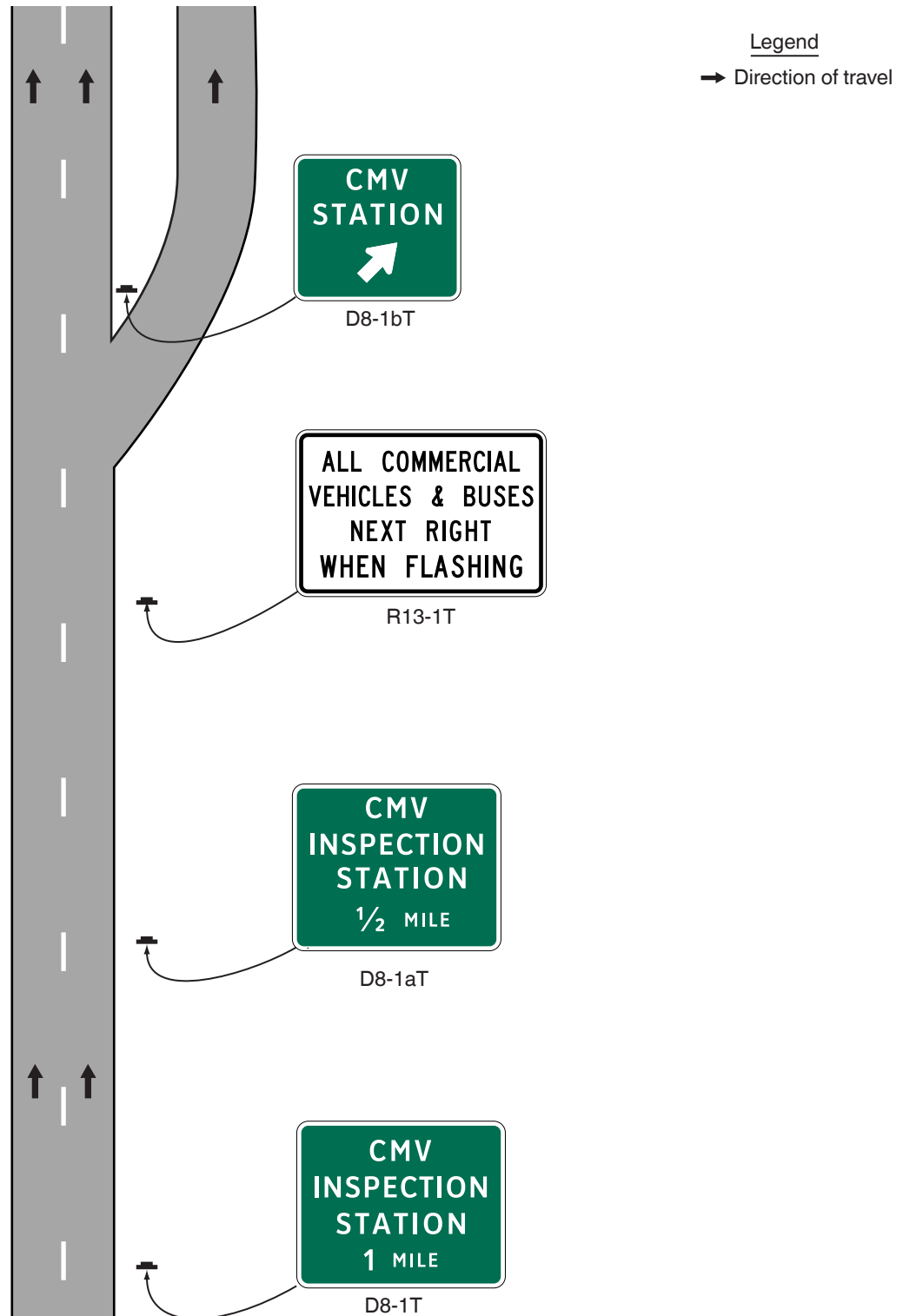
Figure 2D-17TA. Commercial Motor Vehicle (CMV) Inspection Station Signing
