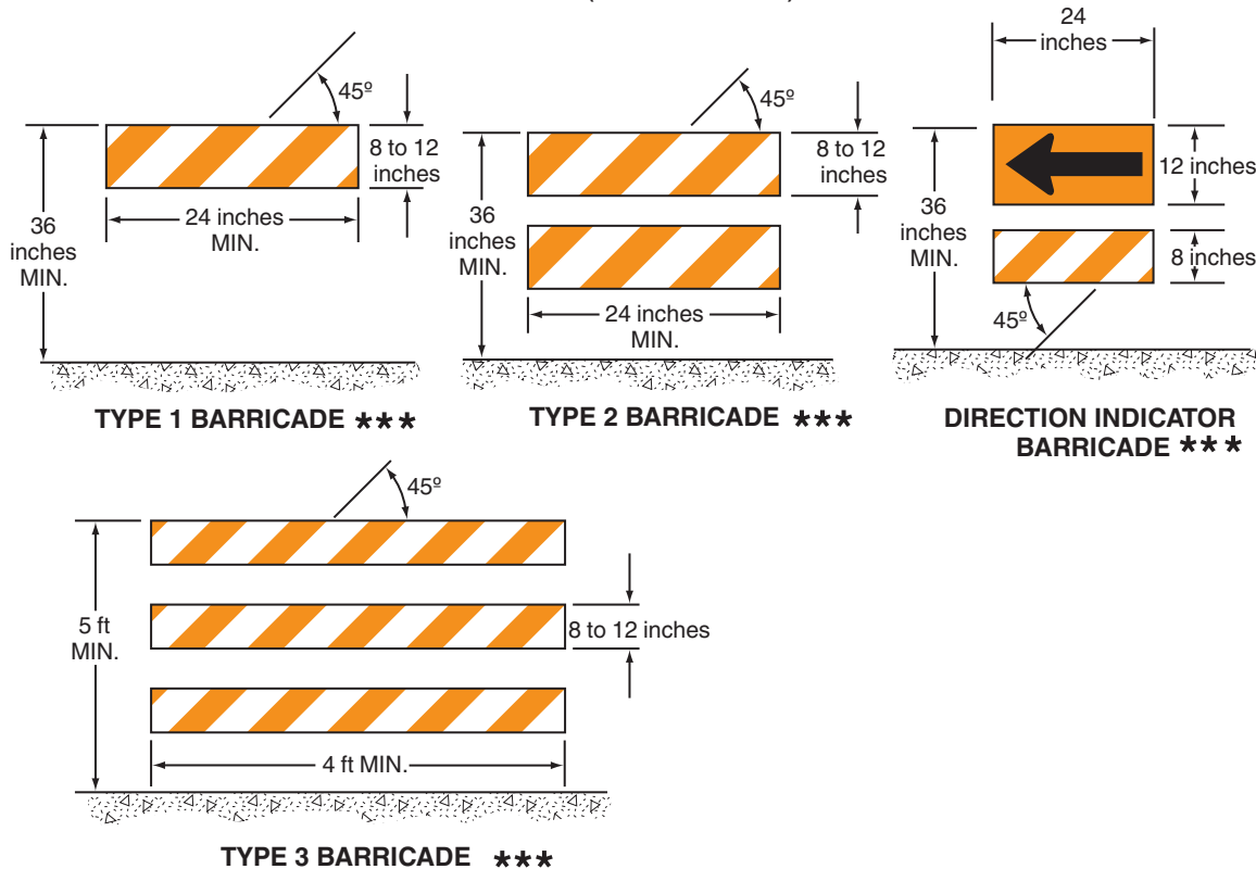
Figure 6F-7. Channelizing Devices (Sheet 2 of 2)
