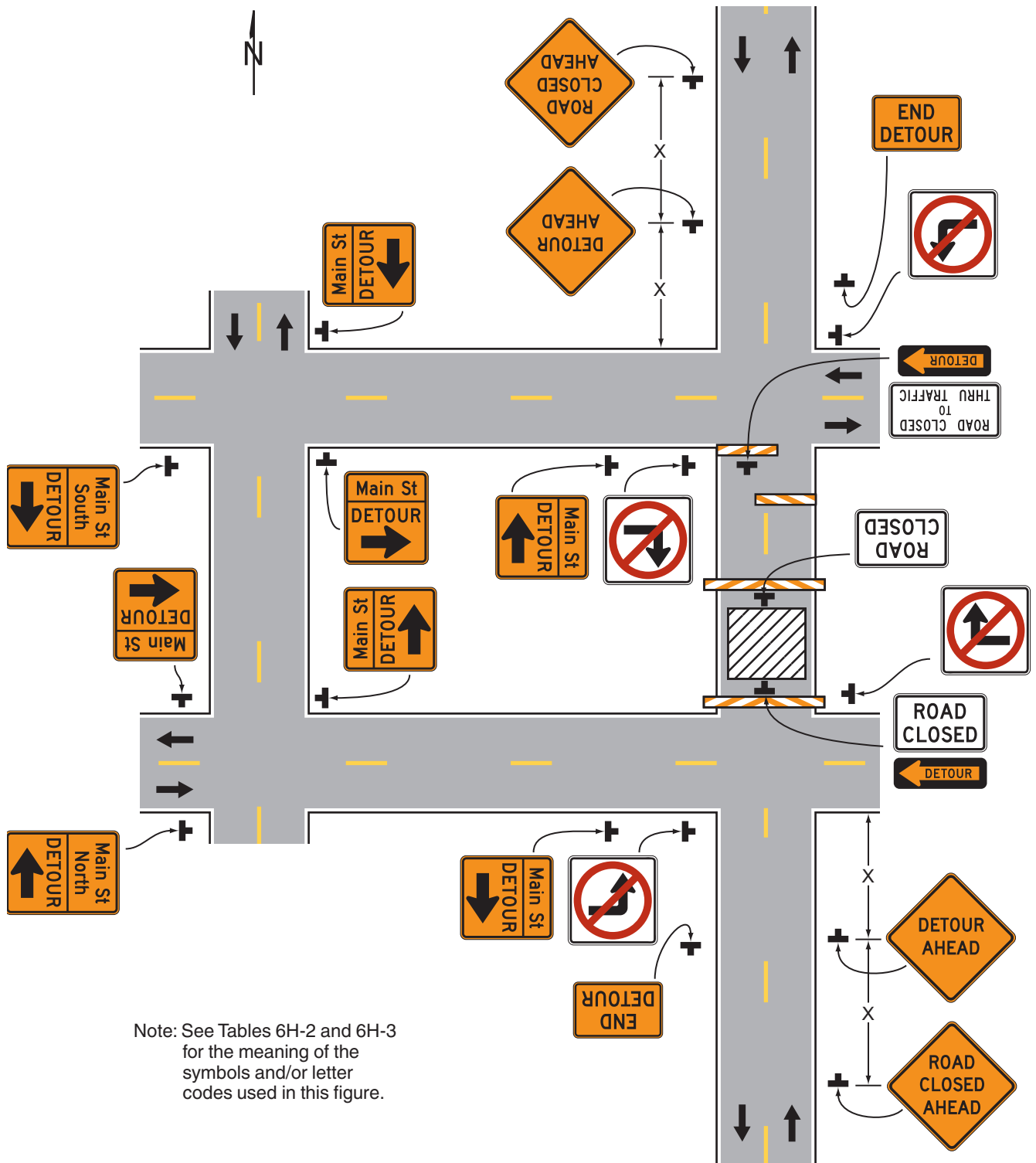
Typical Application 20
