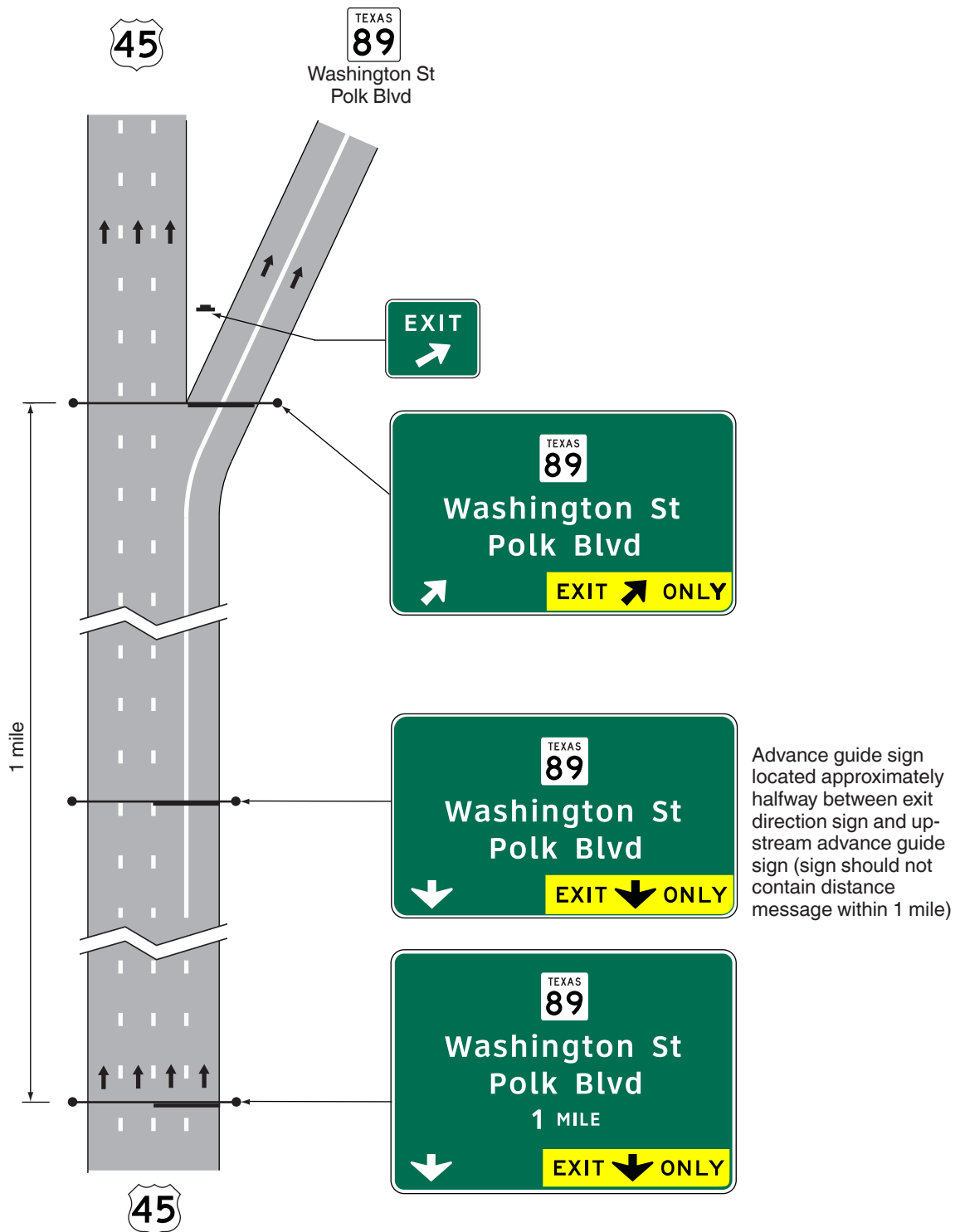
Figure 2E-2TB. Overhead Down Arrow for Option Right Lane Exit
