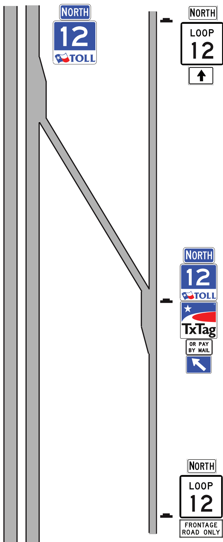
Figure 2F-7TD. Independent Sign Assemblies for Toll Road
