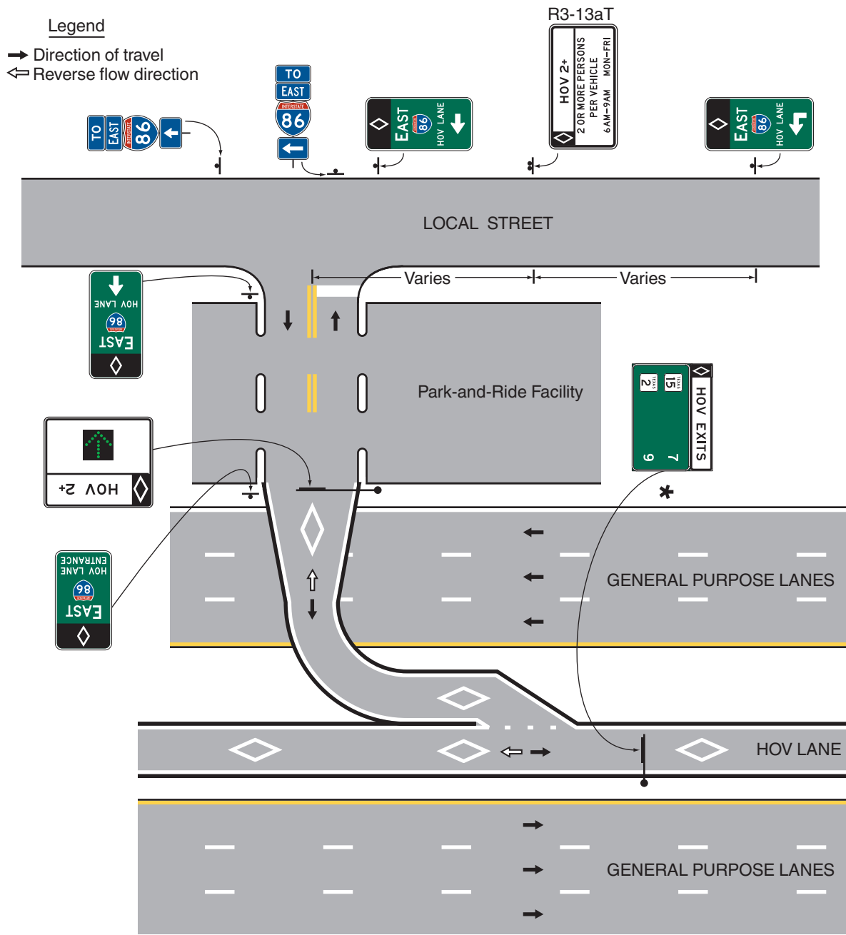
Figure 2G-13. Example of Signing for a Direct Entrance Ramp to an HOV Lane from a Park-and-Ride Facility and a Local Street
