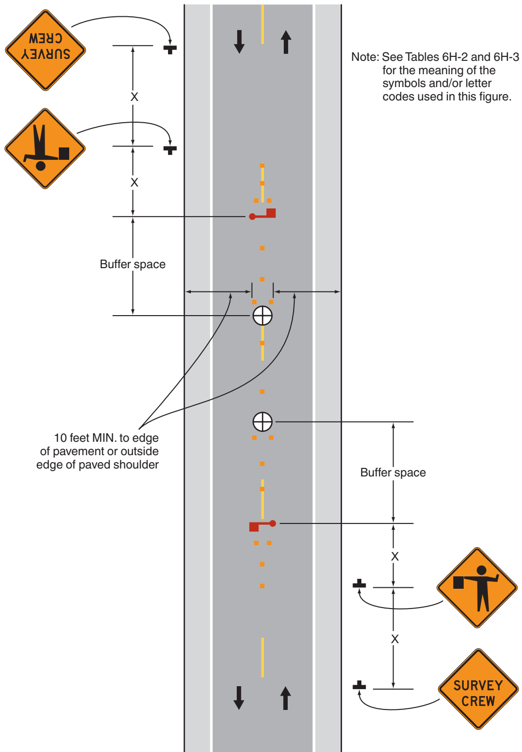
Typical Application 16
