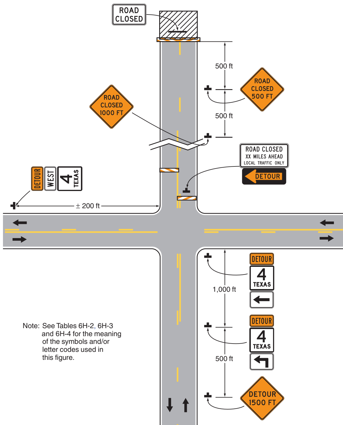
Typical Application 8
