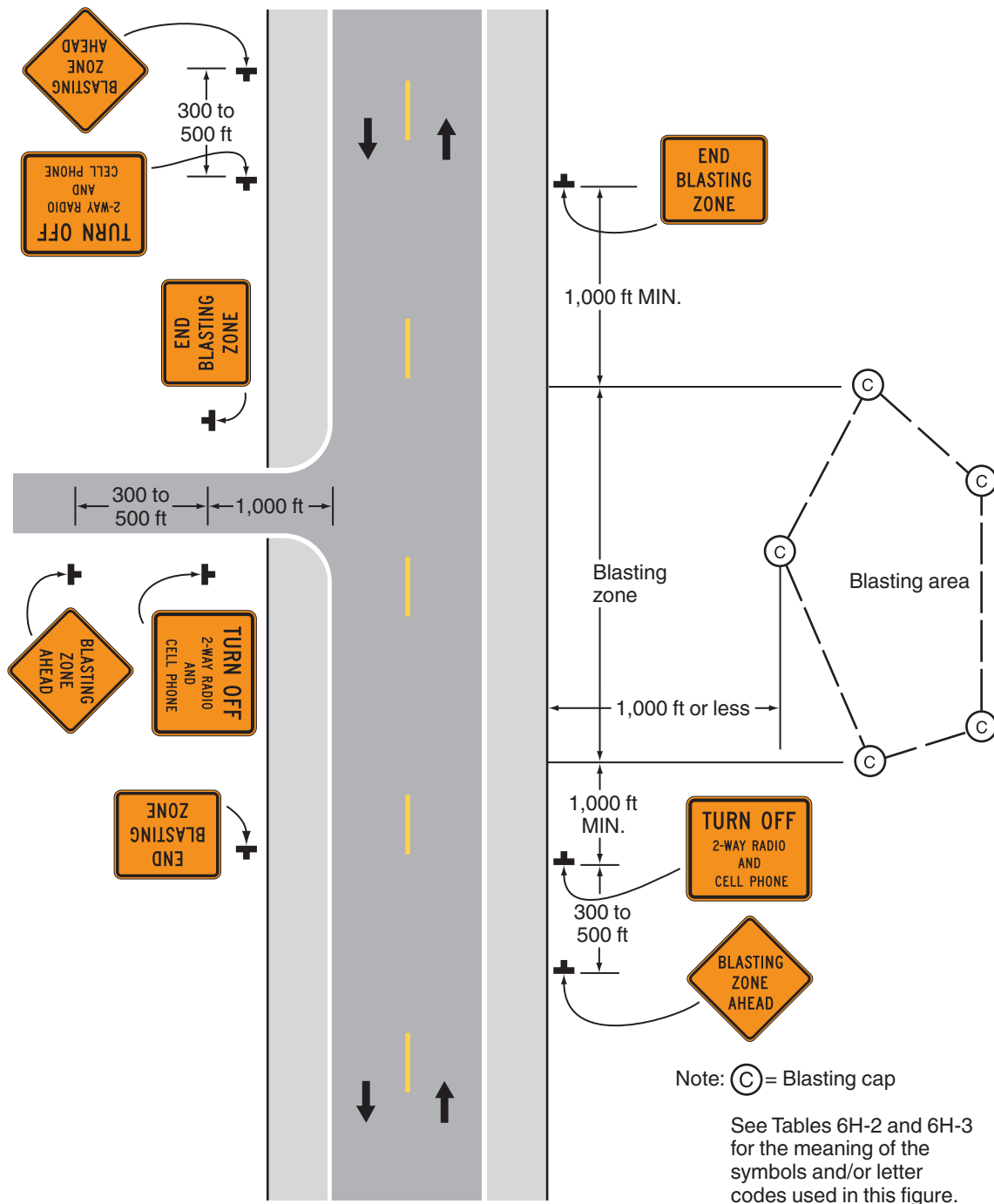
Typical Application 2
