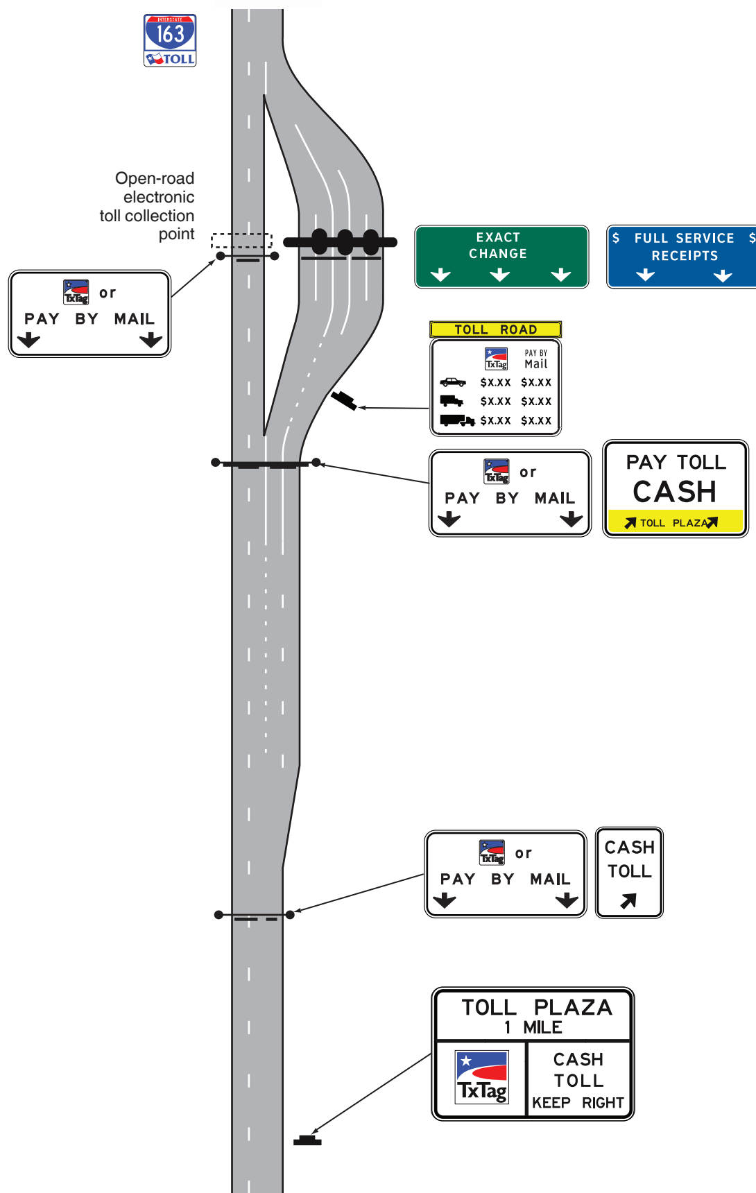
Figure 2F-10TB. Examples of Guide Signs for a Mainlane Toll Plaza on a Diverging Alignment from Open-Road ETC Lanes with Video Billing
