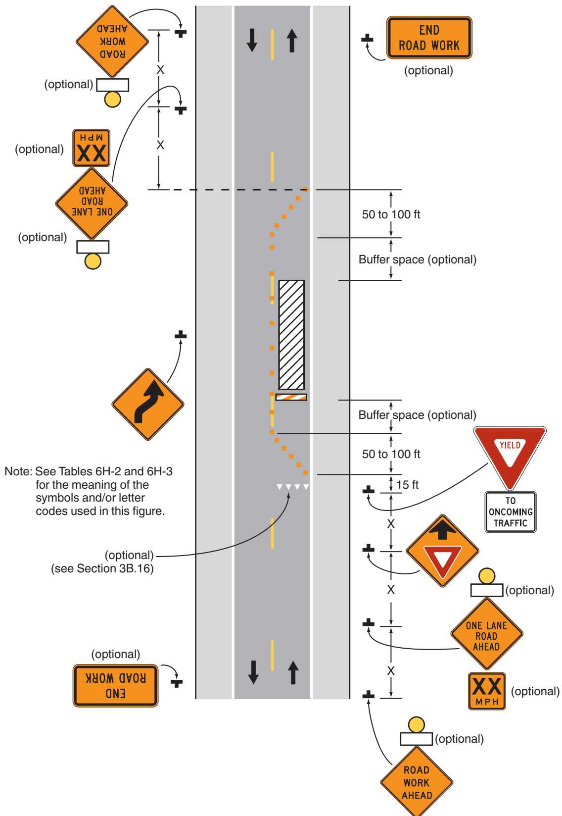
Typical Application 11
