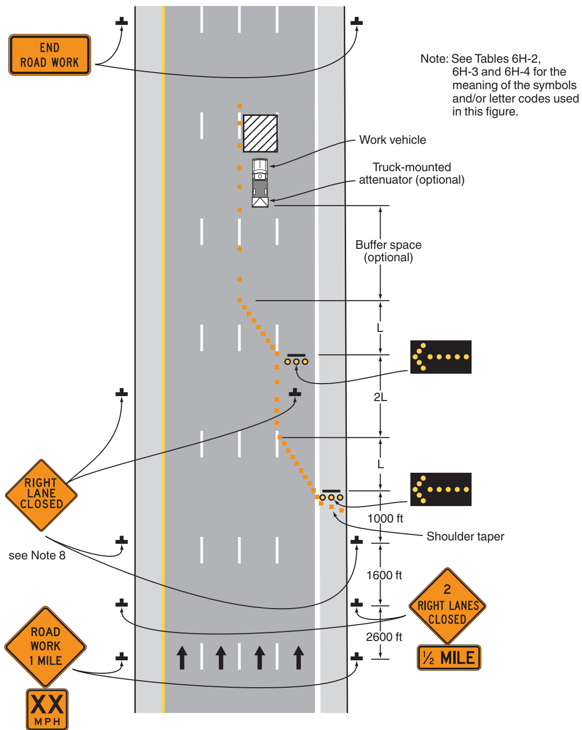
Typical Application 37
